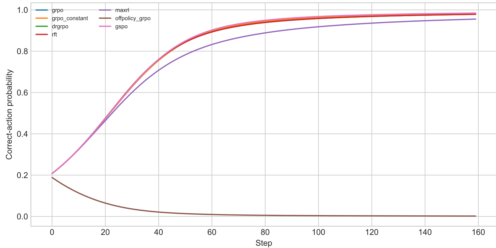
Policy improvement
