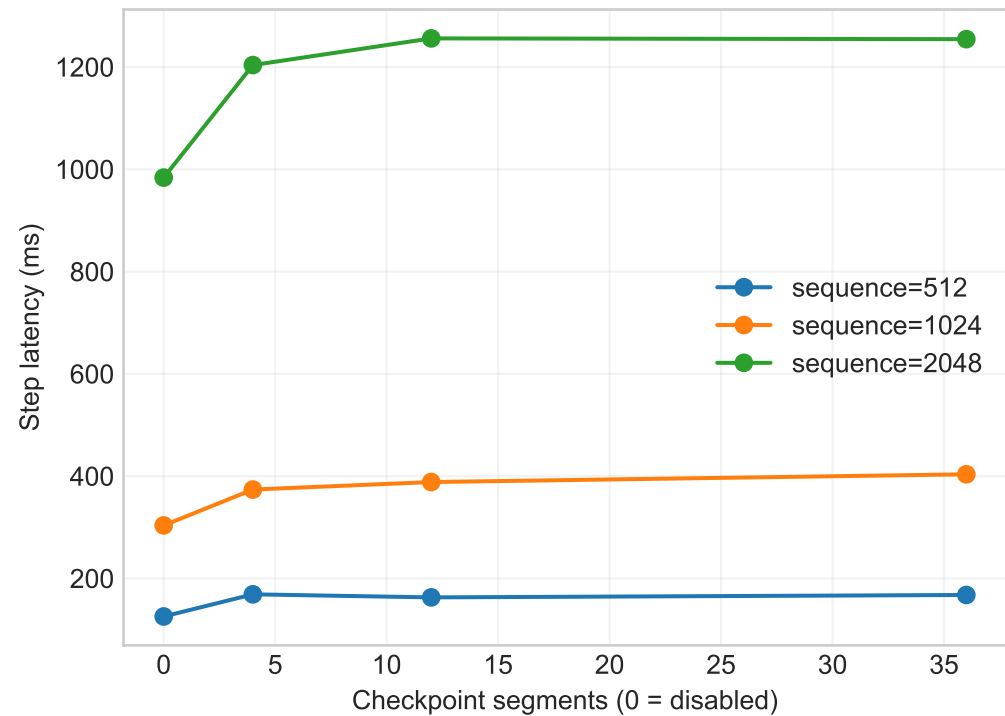
Checkpoint recomputation cost
