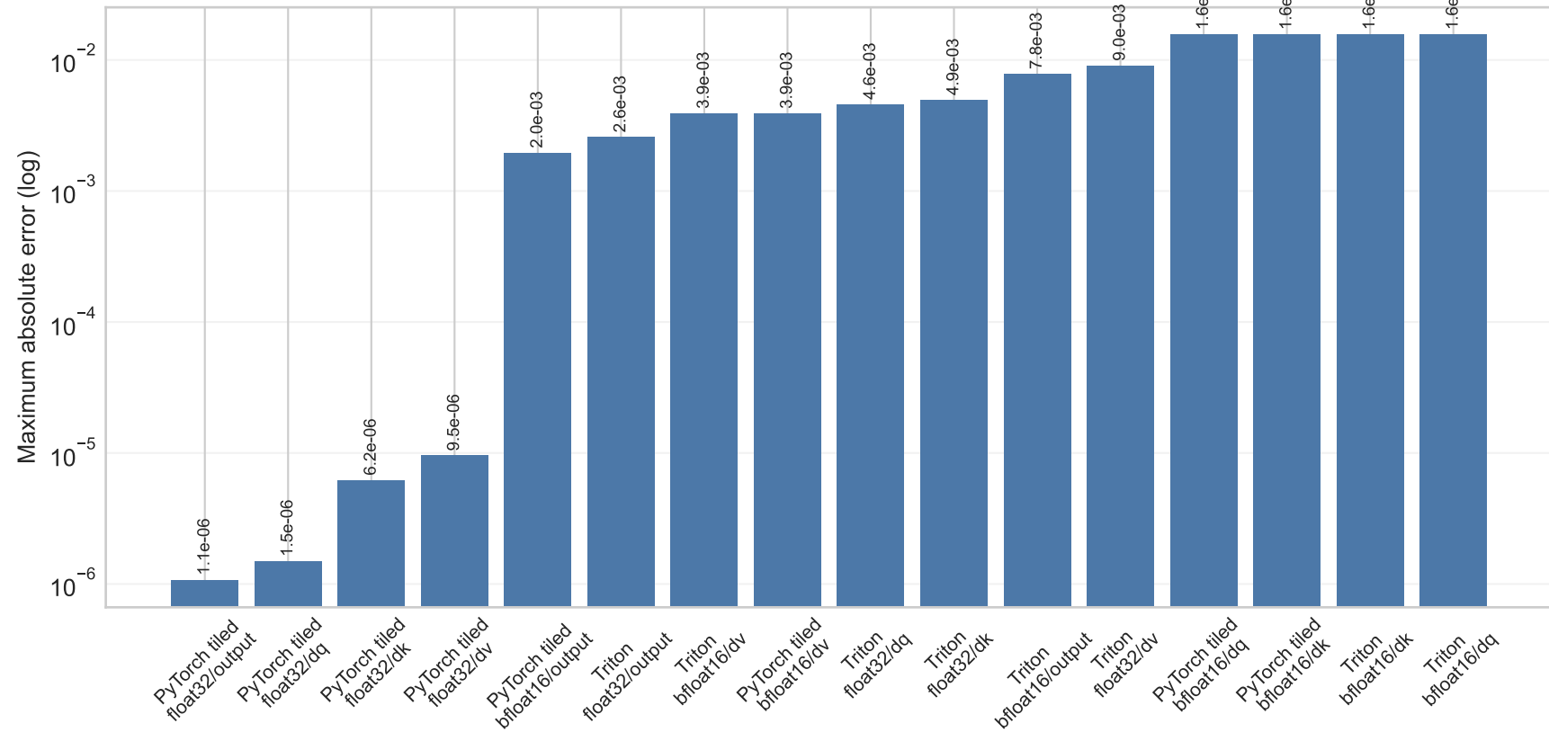
Attention numerical-error envelope
