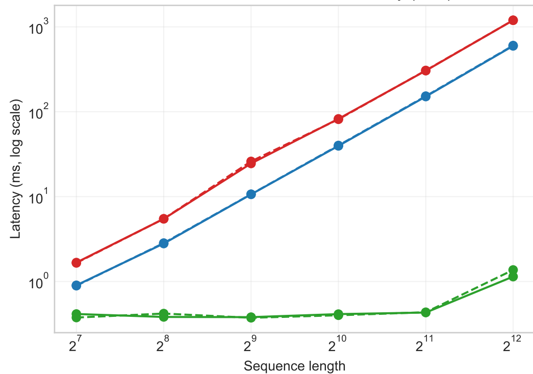
Attention forward + backward latency (bf16)
