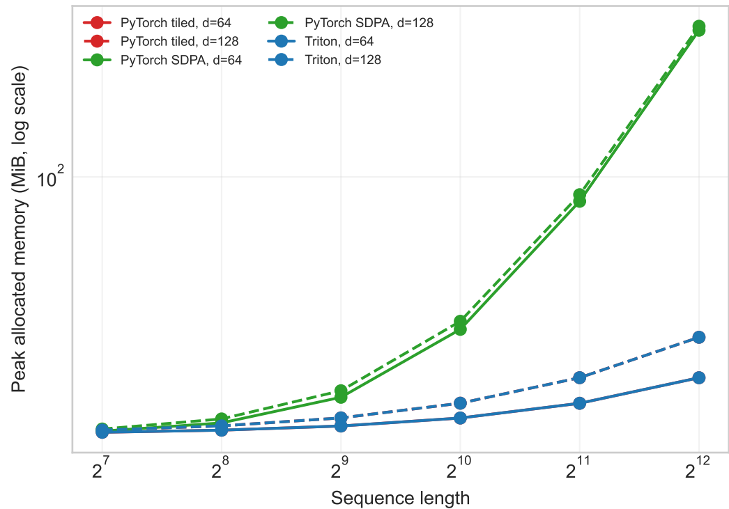
Attention forward + backward memory (fp32)
