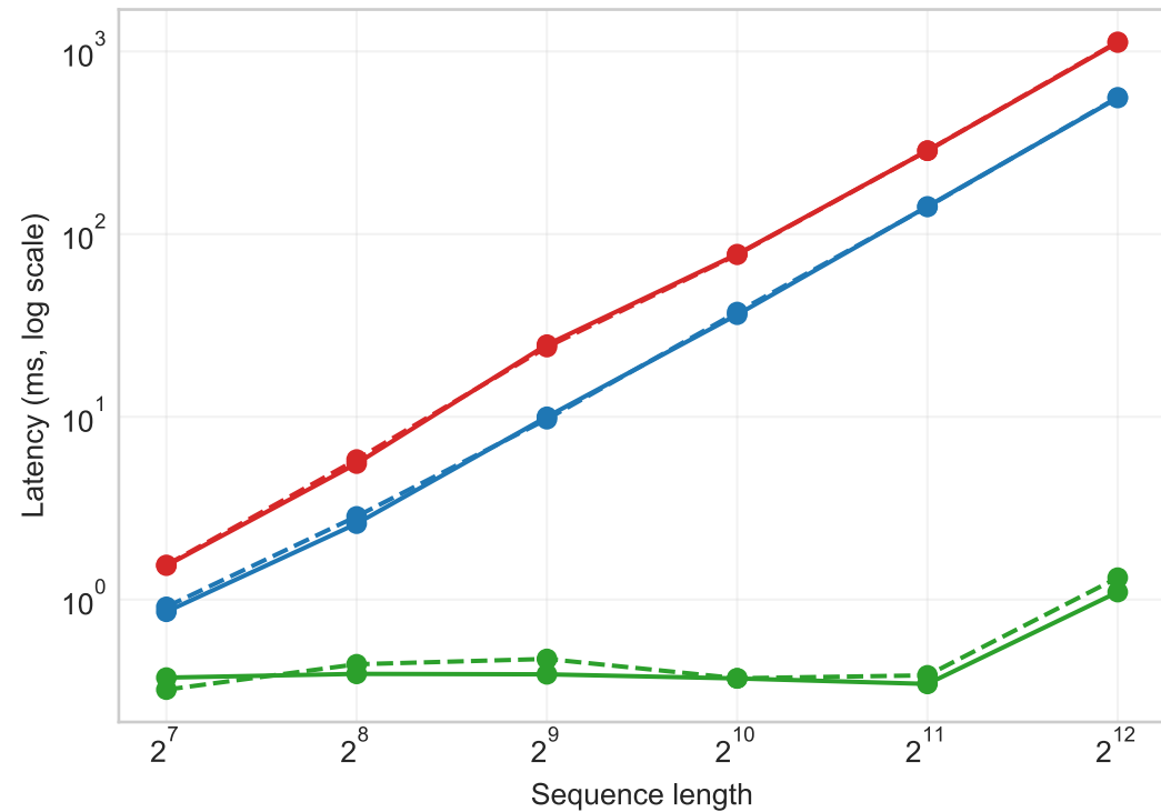
Attention forward + backward latency (fp32)
