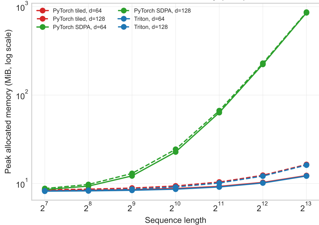
Attention forward memory (bf16)
