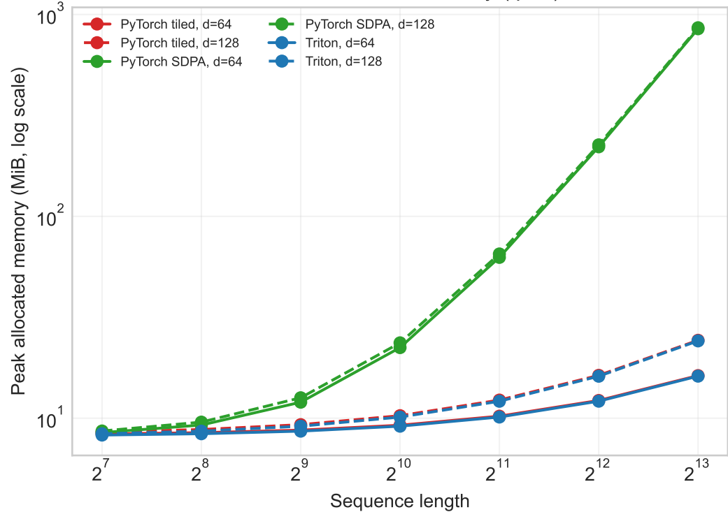
Attention forward memory (fp32)
