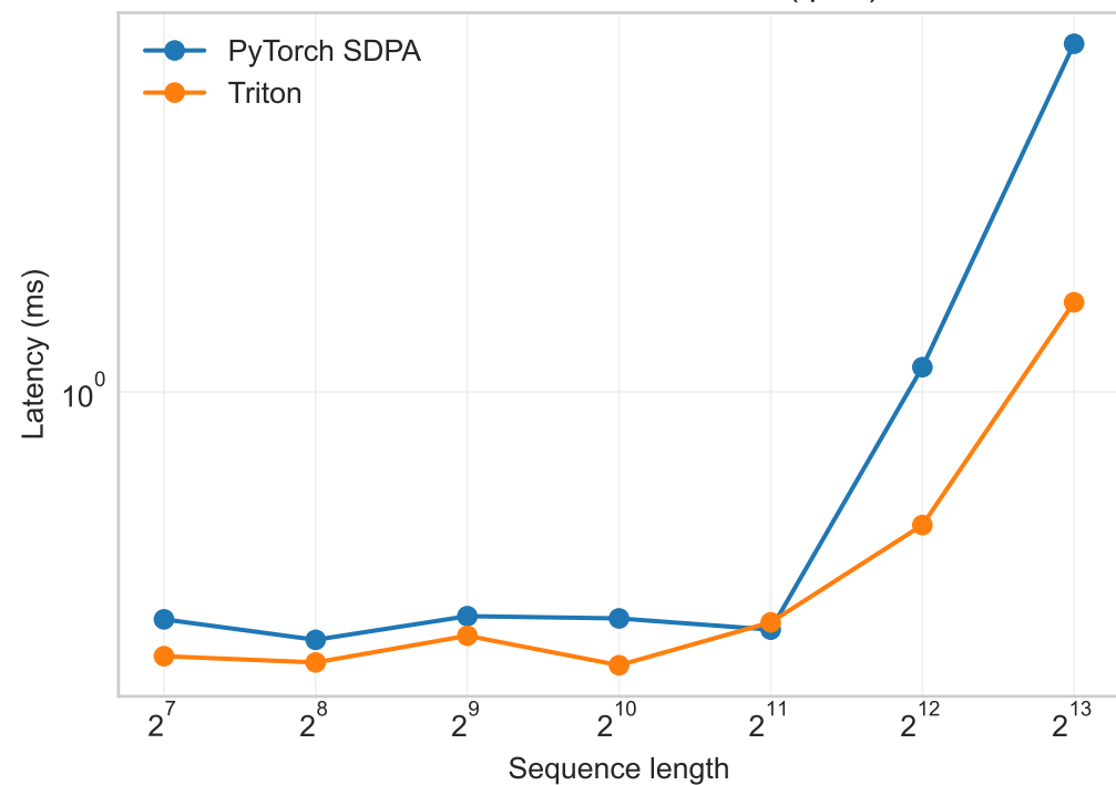
Fused forward + backward (fp32)
