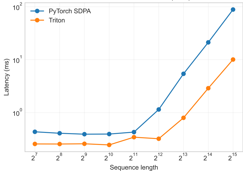
Fused forward + backward (bf16)
