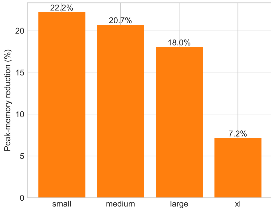
BF16 memory reduction
