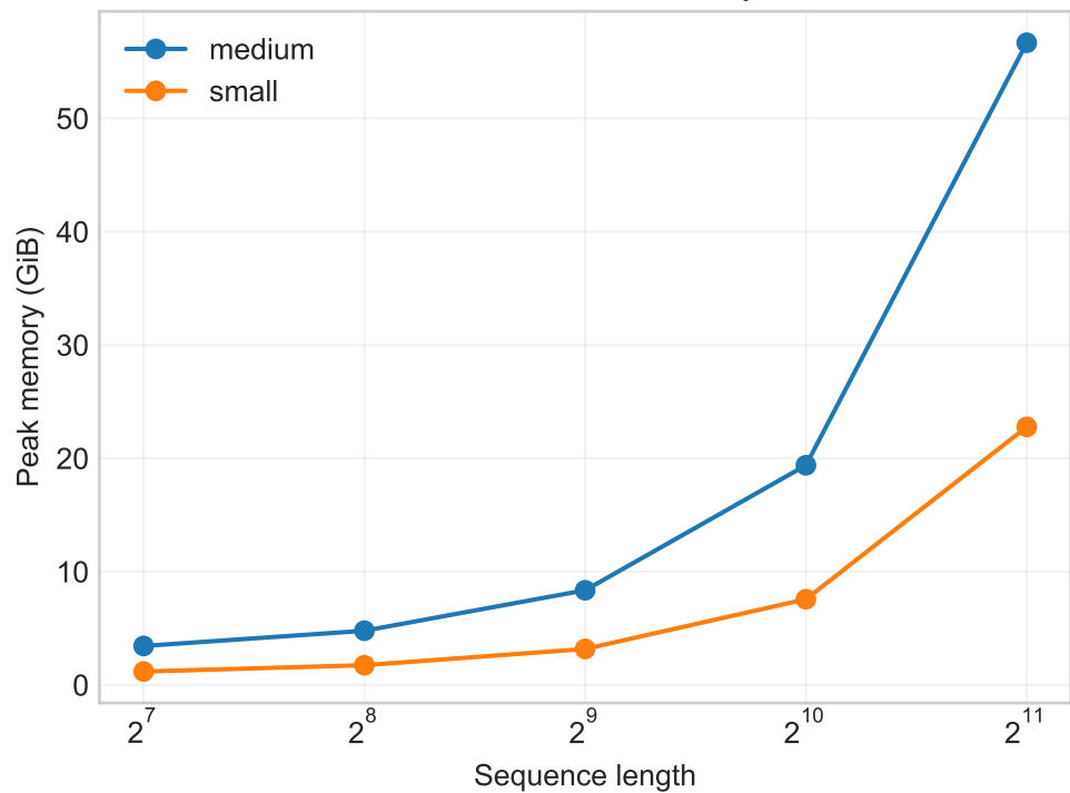
BF16 context memory
