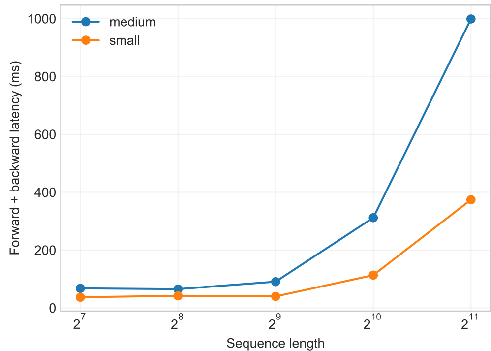
BF16 context scaling
