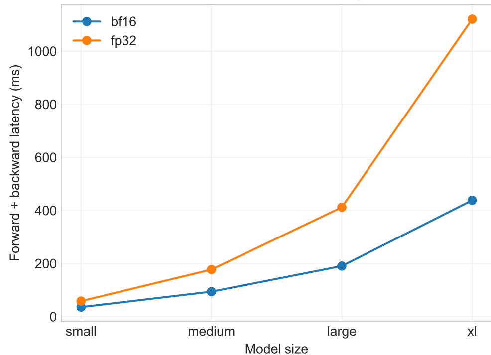
Transformer step latency
