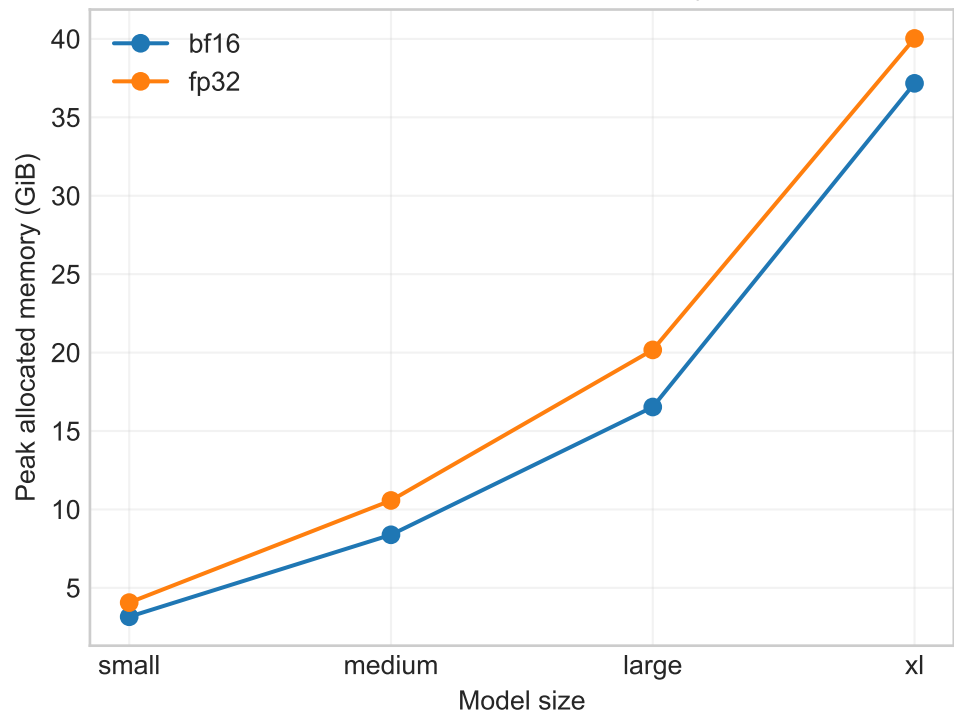
Transformer peak memory
