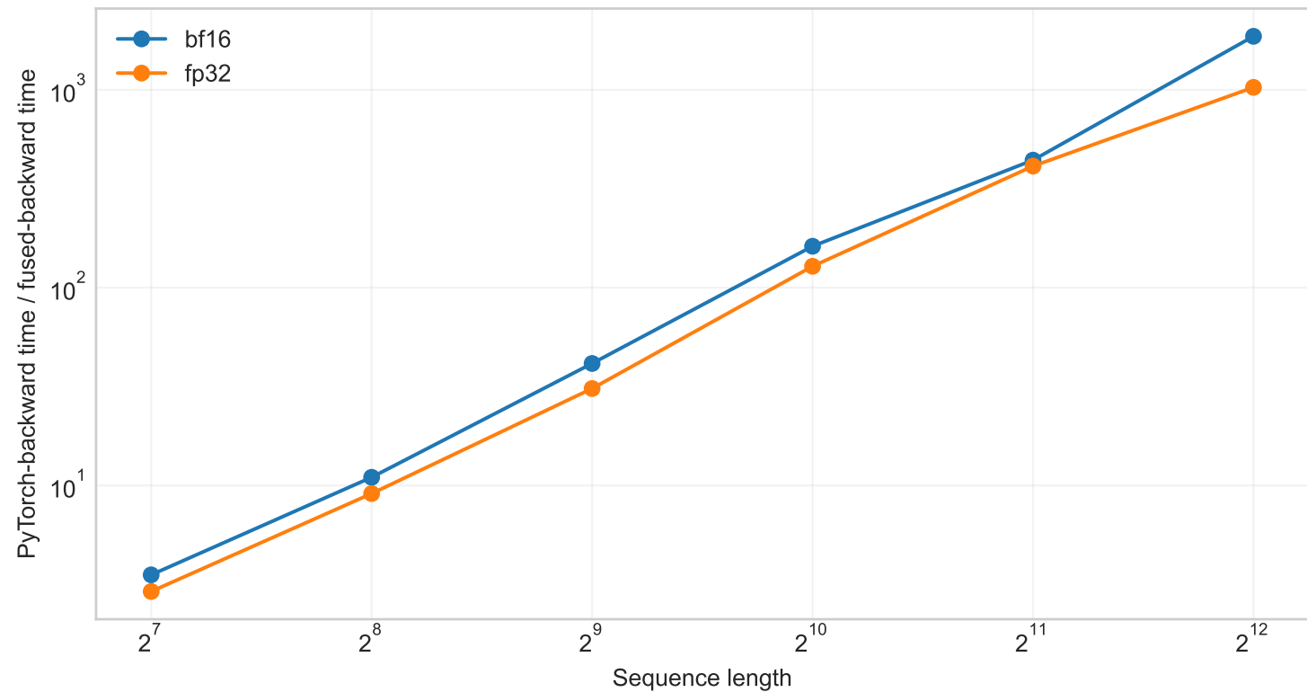
Triton backward fusion speedup
