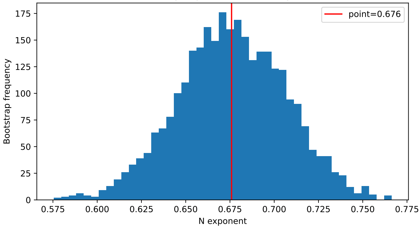
Proxy exponent uncertainty
