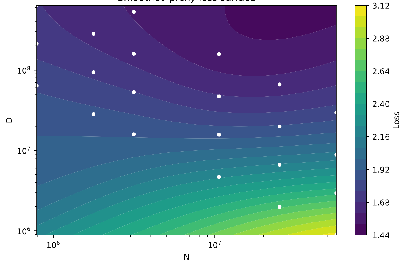
Smoothed proxy loss surface
