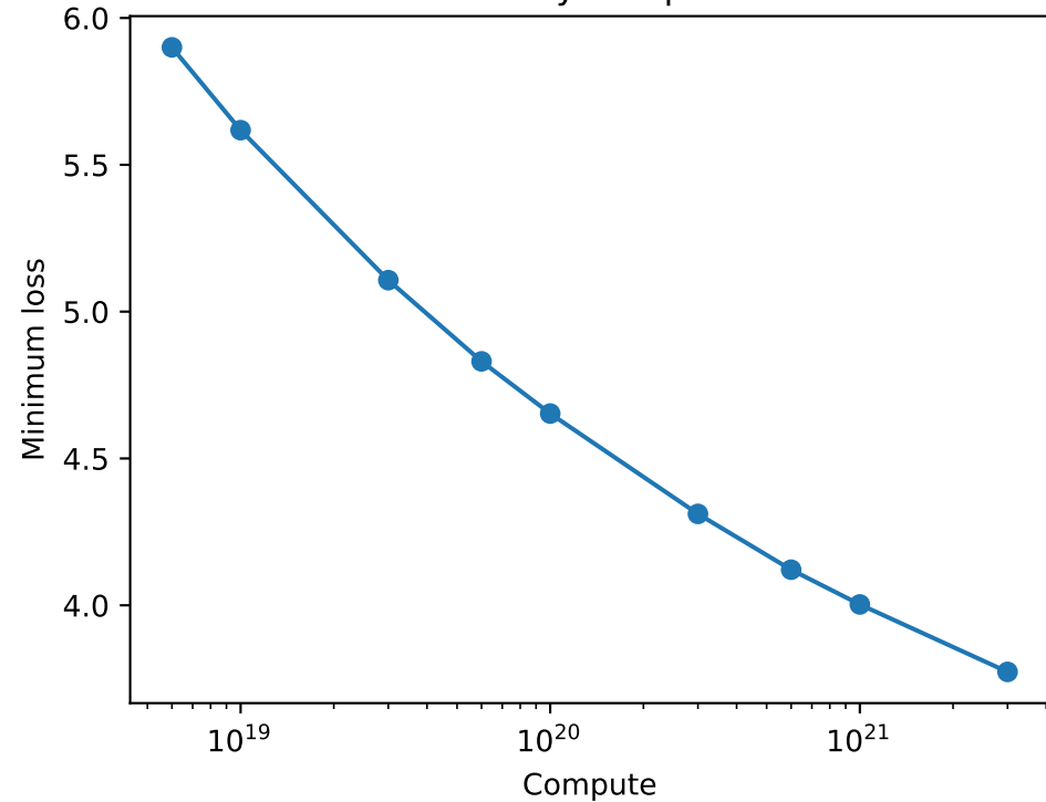
Best loss by compute tier
