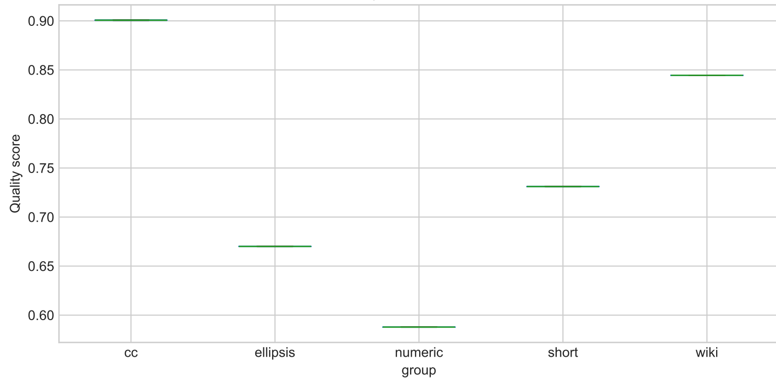
Quality-score distribution
