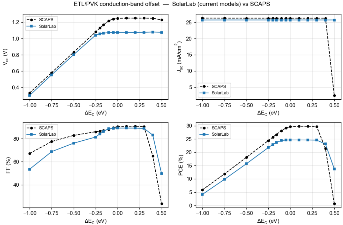
Figure 1: Figure 1. ETL/PVK conduction-band offset ( \Delta E_C ).
