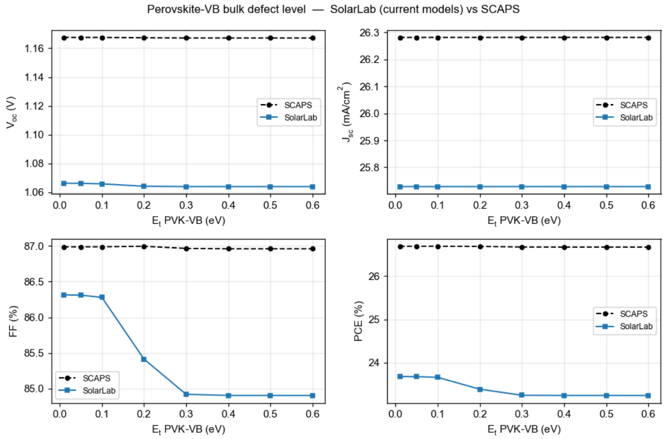
Figure 9: Figure 9. Perovskite valence-band bulk defect level ( E_t ).
