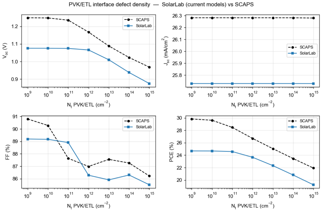
Figure 2: Figure 2. PVK/ETL interface defect density ( N_t ).
