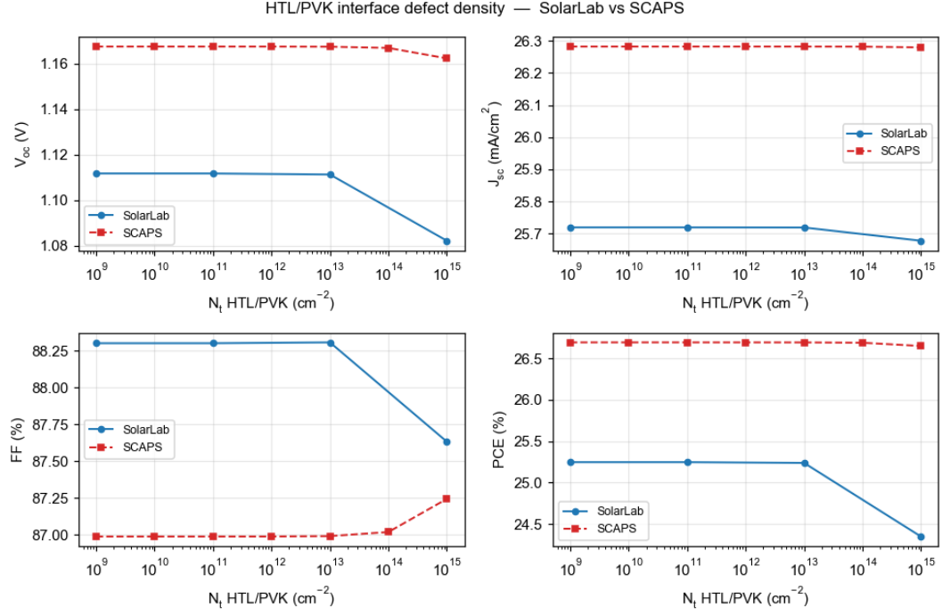
Figure 4: HTL/PVK interface defect density ( N_t ).
