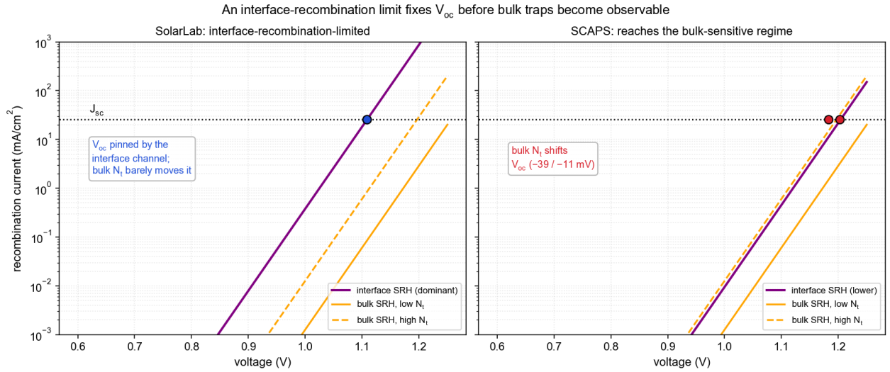
Figure 5: Interface-recombination limit (unchanged from the previous analysis). The SolarLab balance point sits below the bulk-sensitive regime; SCAPS's lower interface component resolves the small bulk responses.
