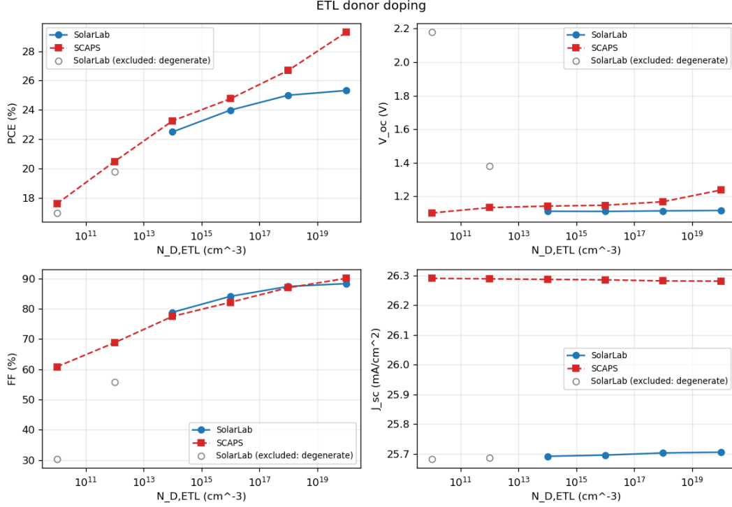
Figure 3: ETL donor-doping sweep, corrected configuration. Degenerate low-doping points (extracted V_{oc} at or above the detailed-balance ceiling) are excluded from the statistics and shown as grey open markers; the well-posed arm ( N_D \geq 10^{14} \text{ cm}^{-3} ) matches SCAPS in direction.
