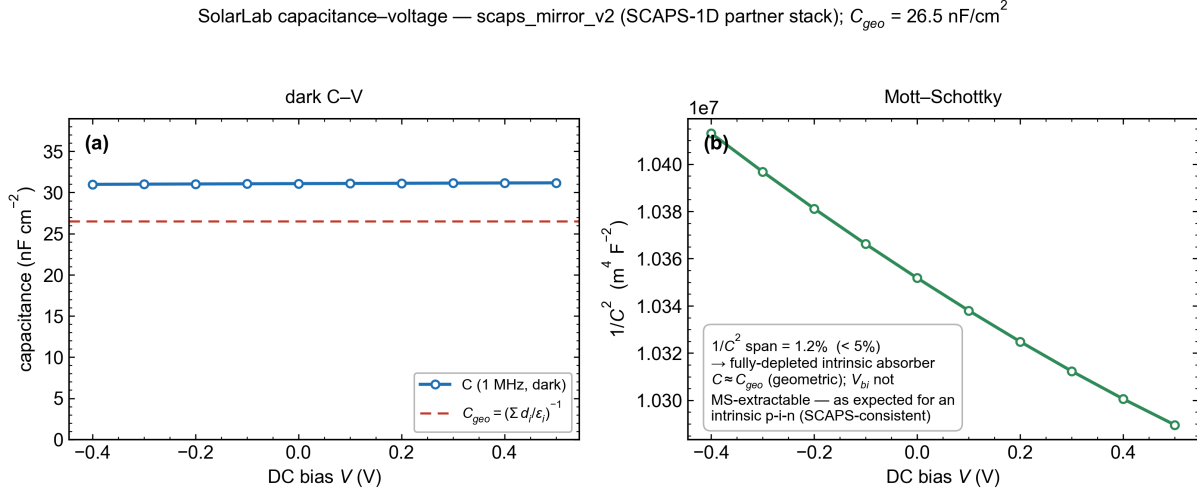
Figure 7: (a) Dark capacitance–voltage at 1 MHz with the geometric series capacitance C_{geo} for reference. (b) Mott–Schottky plot, 1/C^2 versus bias.
