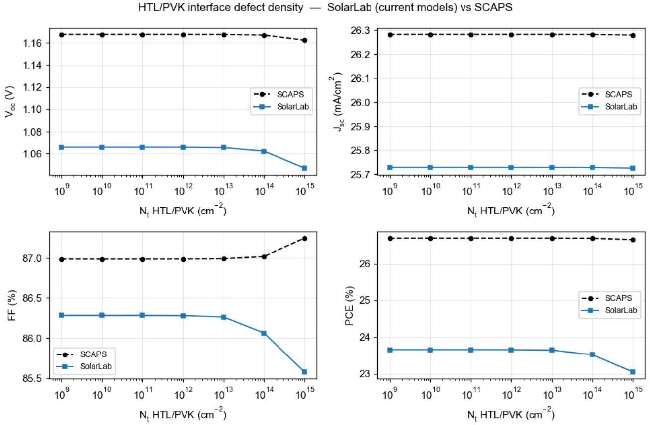
Figure 4: HTL/PVK interface defect density ( N_t ).
