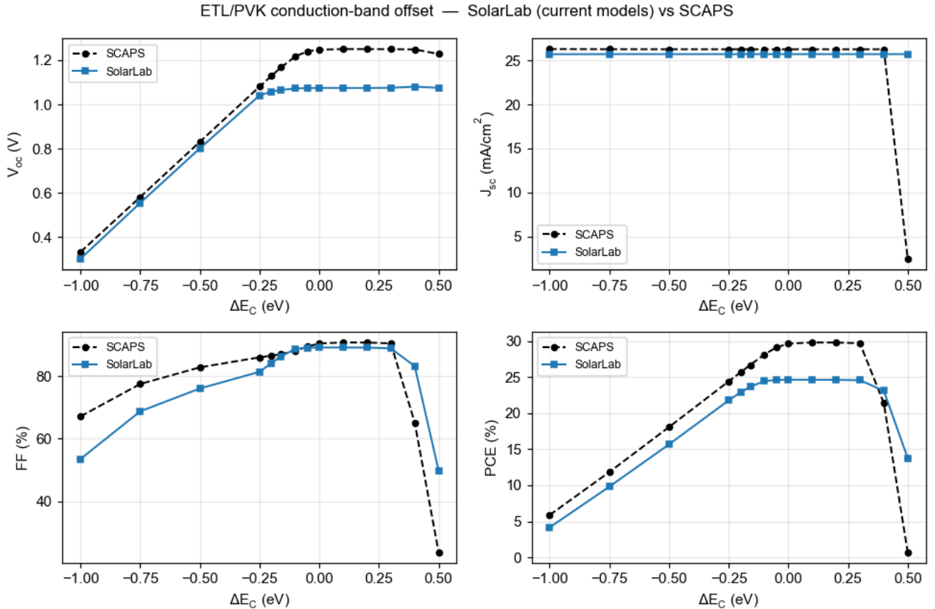
Figure 1: ETL/PVK conduction-band offset ( \Delta E_C ).
