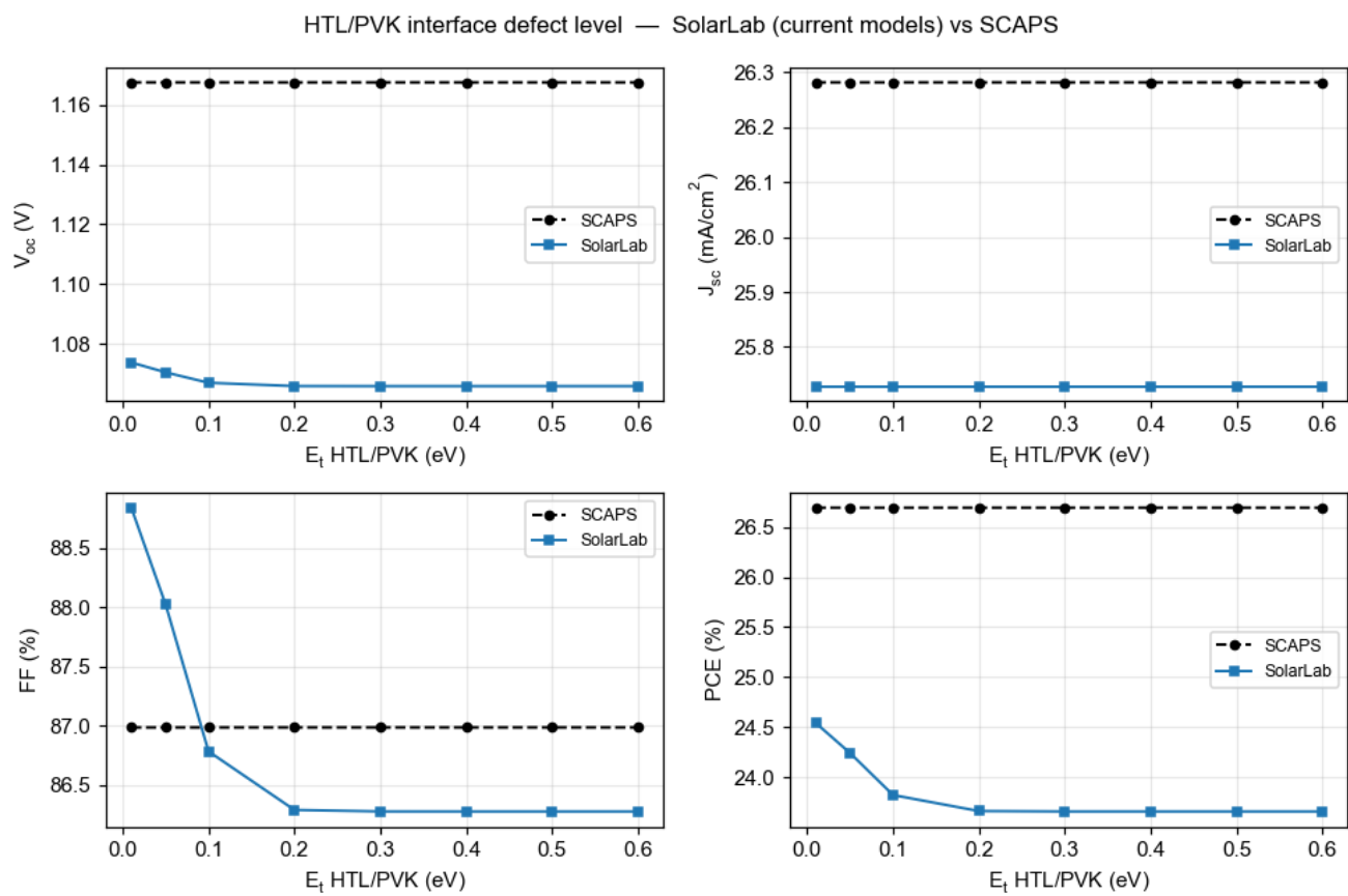
Figure 10: HTL/PVK interface defect level ( E_t ).
