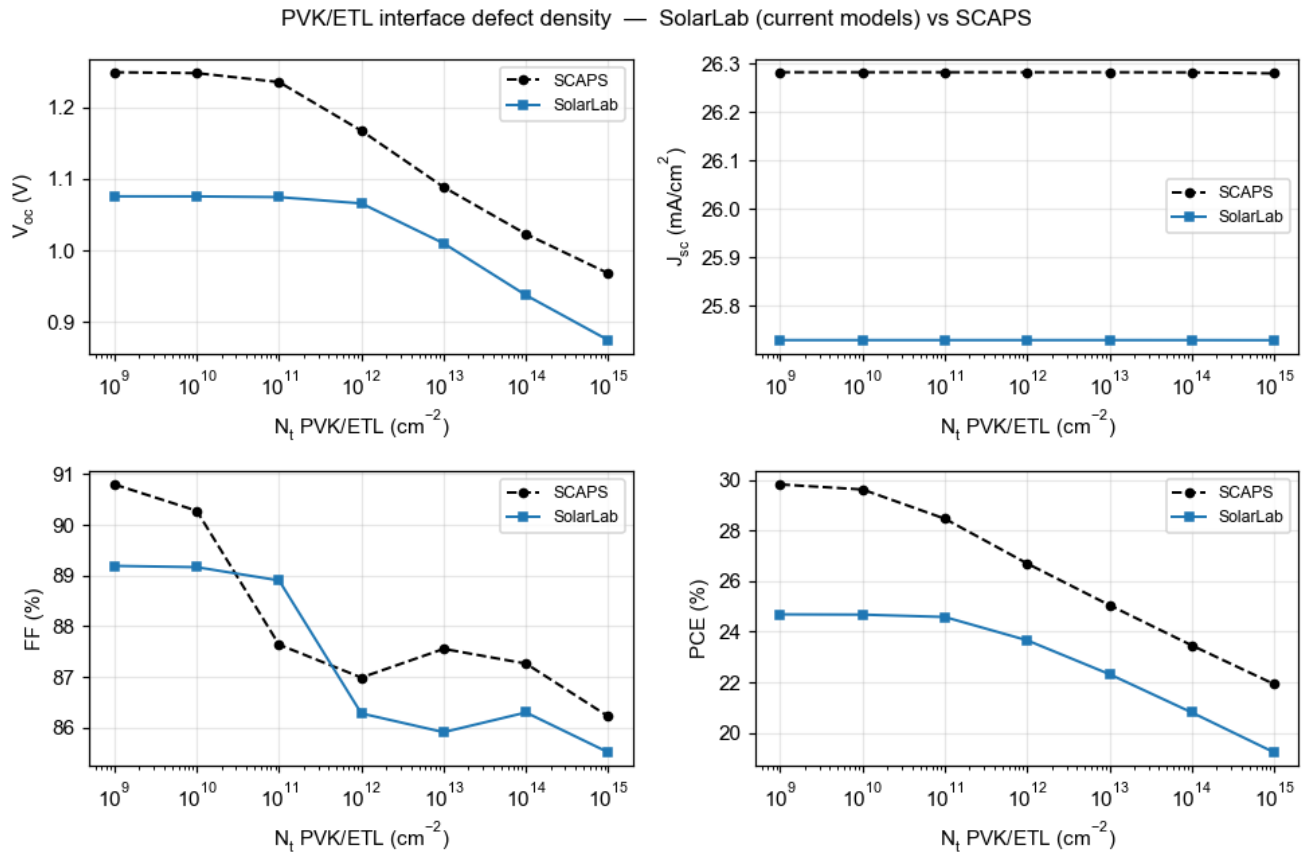
Figure 2: PVK/ETL interface defect density ( N_t ).
