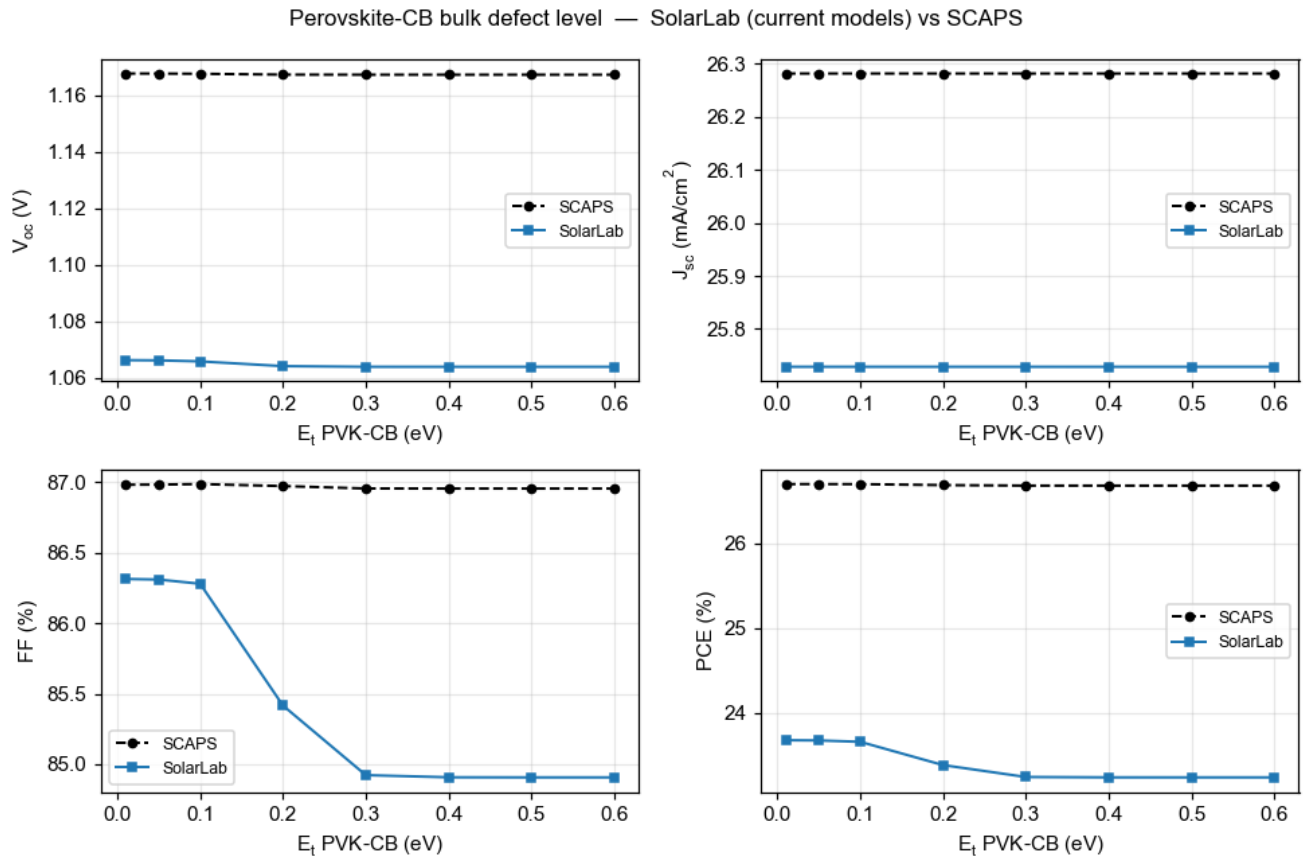
Figure 8: Perovskite conduction-band bulk defect level ( E_t ).
