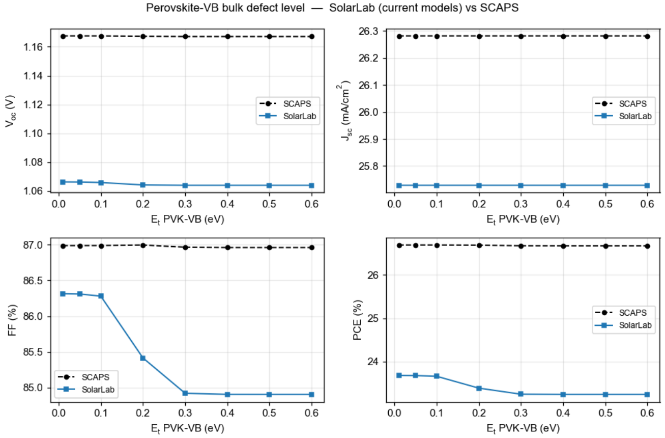
Figure 9: Perovskite valence-band bulk defect level ( E_t ).
