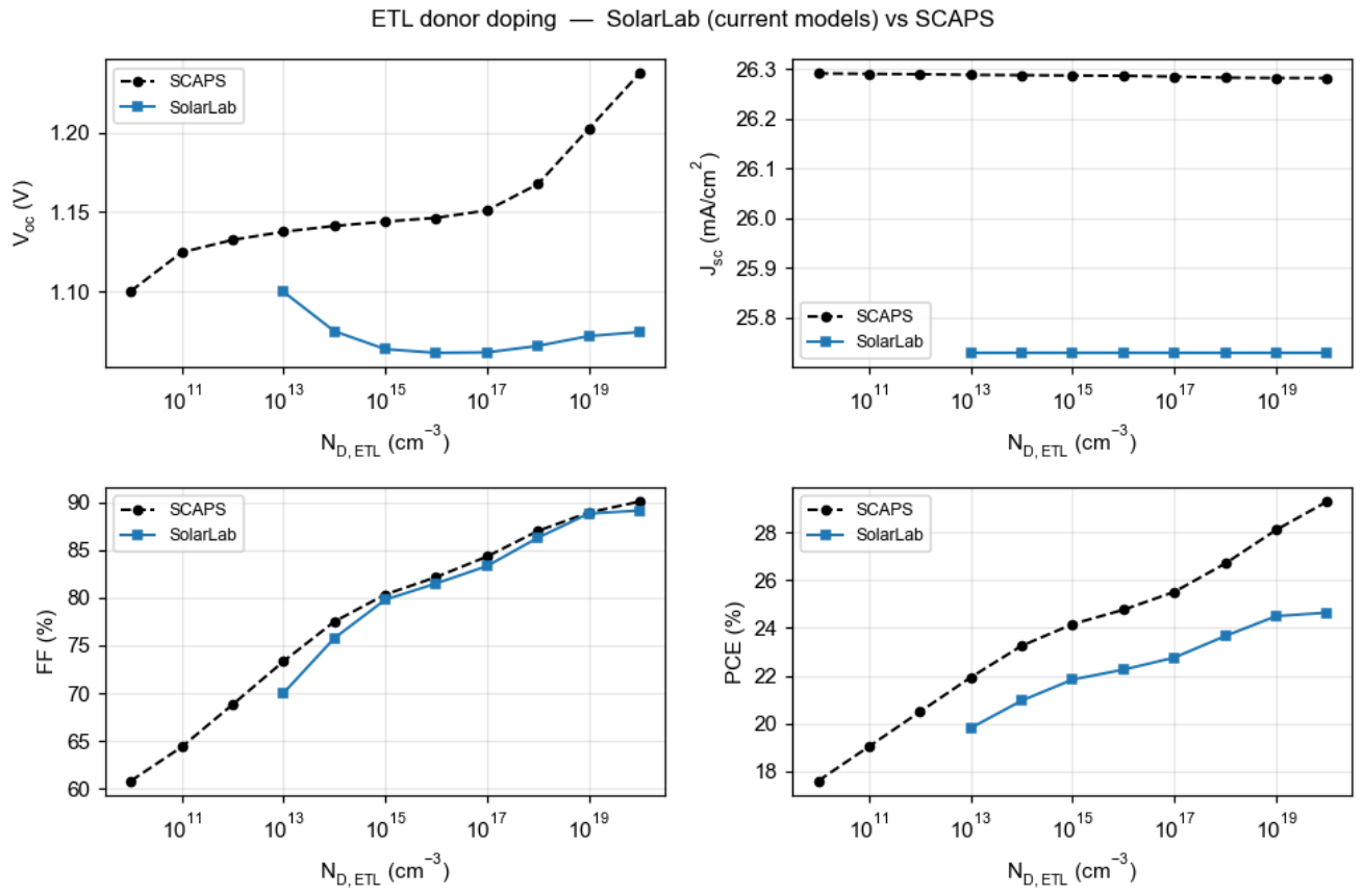
Figure 5: ETL donor doping (ND).
