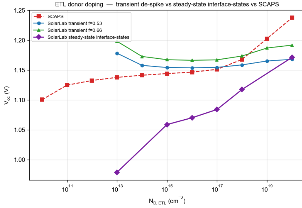
Figure 12: ETL donor doping V_{oc} : the transient de-spike curves ( f=0.53 blue, f=0.66 green) are U-shaped — direction mismatch — while the steady-state interface-states driver (purple) rises monotonically with doping, matching the SCAPS direction. Magnitude over-responds and the absolute sits below SCAPS (the interface-channel calibration residual).
