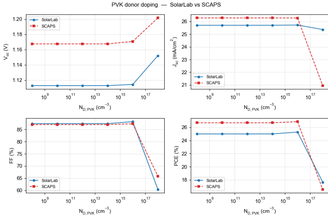
Figure 11: PVK donor doping ( N_{D,PVK} ).
