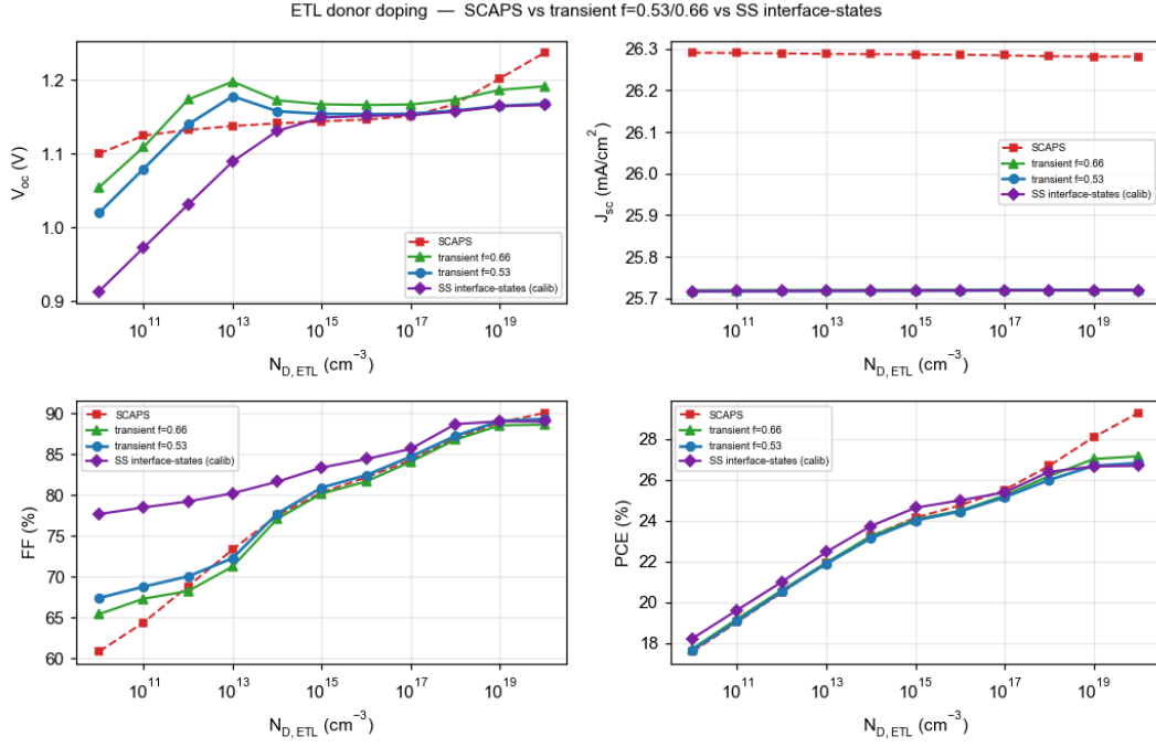
Figure 2: ETL donor doping ( N_D ). Updated 2026-07-02: with the work-function contact-reservoir floor (flat_band_metal_contacts, \phi_B = 0.42 eV) the transient curves now bracket the full doping range and rise with doping at low N_D — the contact starvation that previously left the three lowest points unbracketed / on an unphysical >E_g branch is fixed (RMS 39 mV vs SCAPS at f = 0.53 ); a shallow mid-doping de-spike residual (the \sim 10^{13} – 10^{16} dip) remains. The SS interface-states V_{oc} also rises with doping. All three SolarLab configurations now match the SCAPS rising direction.
