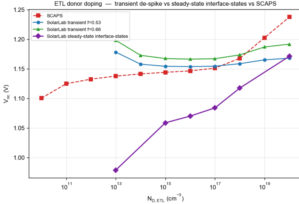
Figure 12: ETL donor doping V_{oc} ( predates the 2026-07-02 contact-reservoir fix — see the update note above and the Section-4 panels for the fixed transient): the transient de-spike curves ( f=0.53 blue, f=0.66 green) are U-shaped — direction mismatch — while the steady-state interface-states driver (purple) rises monotonically with doping, matching the SCAPS direction. Magnitude over-responds and the absolute sits below SCAPS (the interface-channel calibration residual).
