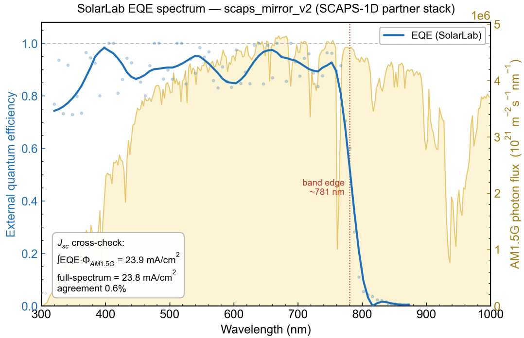
Figure 6: External quantum efficiency EQE(\lambda) (left axis) with the AM1.5G photon flux for context (right axis). The dotted line marks the absorber band edge; the inset reports the consistency check between the AM1.5G-integrated and full-spectrum short-circuit current densities.
