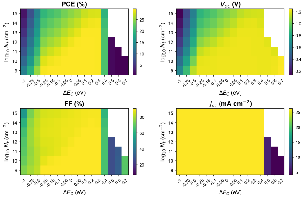
Figure 2: Scan B ( N_t \times \Delta E_C ) on the perovskite/ETL interface. Panels and axes as in Figure 1, with the horizontal axis the conduction-band offset \Delta E_C . White cells in the SCAPS block are grid points the reference solver did not resolve.
