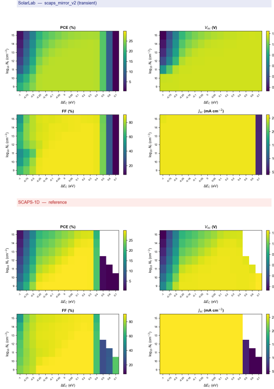
Figure 2: Scan B ( N_t \times \Delta E_C ) on the perovskite/ETL interface. Panels and axes as in Figure 1, with the horizontal axis the conduction-band offset \Delta E_C . White cells in the SCAPS block are grid points the reference solver did not resolve.
