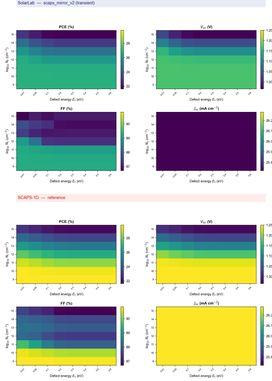
Figure 1: Scan A ( N_t \times E_t ) on the perovskite/ETL interface. SolarLab (upper block) and SCAPS-1D (lower block) four-panel maps of PCE, V_{oc} , FF and J_{sc} ; the vertical axis is \log_{10} N_t and the horizontal axis is the trap energy E_t .
