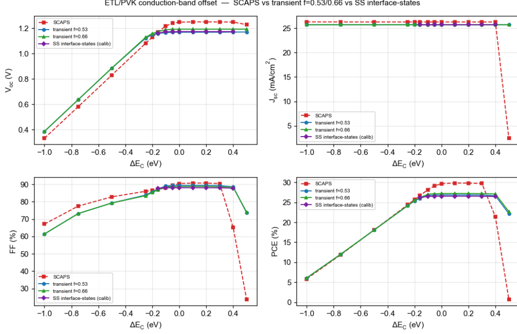
Figure 1: ETL/PVK conduction-band offset ( \Delta E_C ). The SS-states curve (purple) covers the flat-band operative region ( \Delta E_C \geq -0.16 eV, 8 of 14 points), where it sits directly on the transient curves — CBO is a band-offset effect, so SS approx the transient (not interface-limited). The deep-CBO points ( \Delta E_C \leq -0.2 eV) collapse V_{oc} below ~1.1 V and destroy the junction: the SS interface-states Newton cannot converge there (>60 s/point), so those points carry only the transient/SCAPS series.
