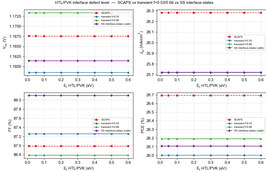
Figure 10: HTL/PVK interface defect level ( E_t ).
