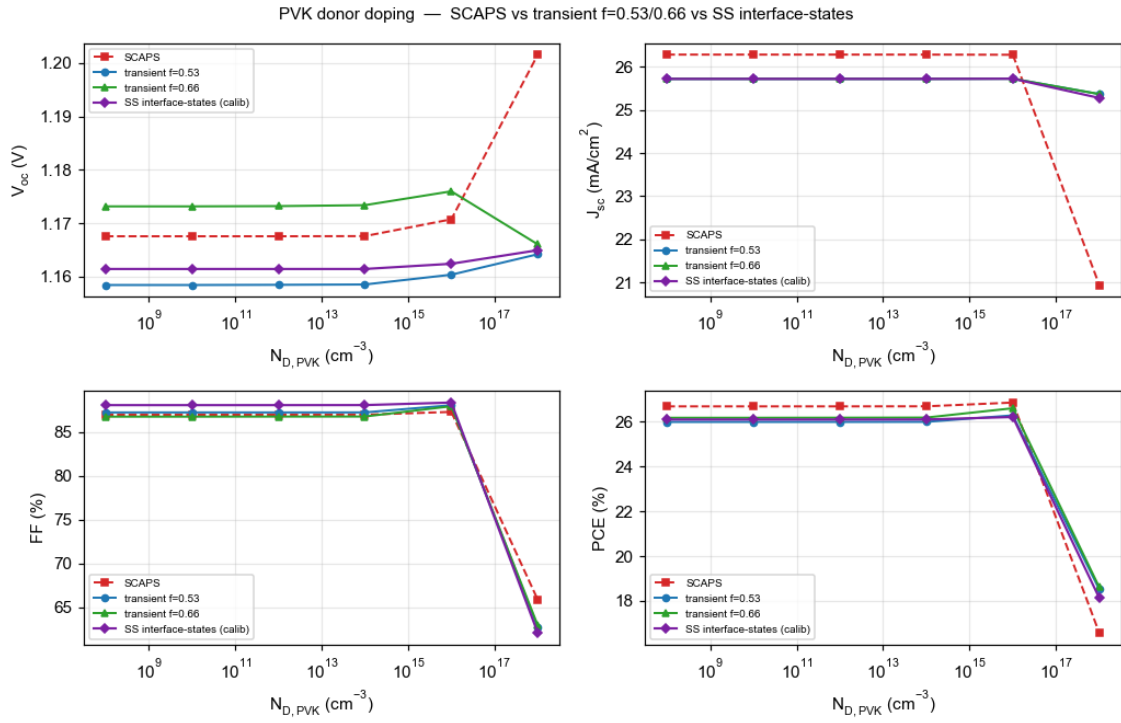
Figure 3: PVK donor doping ( N_{D,PVK} ).
