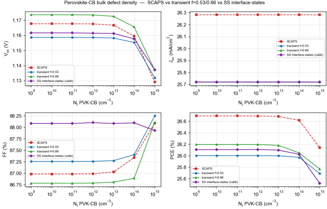
Figure 4: Perovskite-CB bulk defect density ( N_t ).
