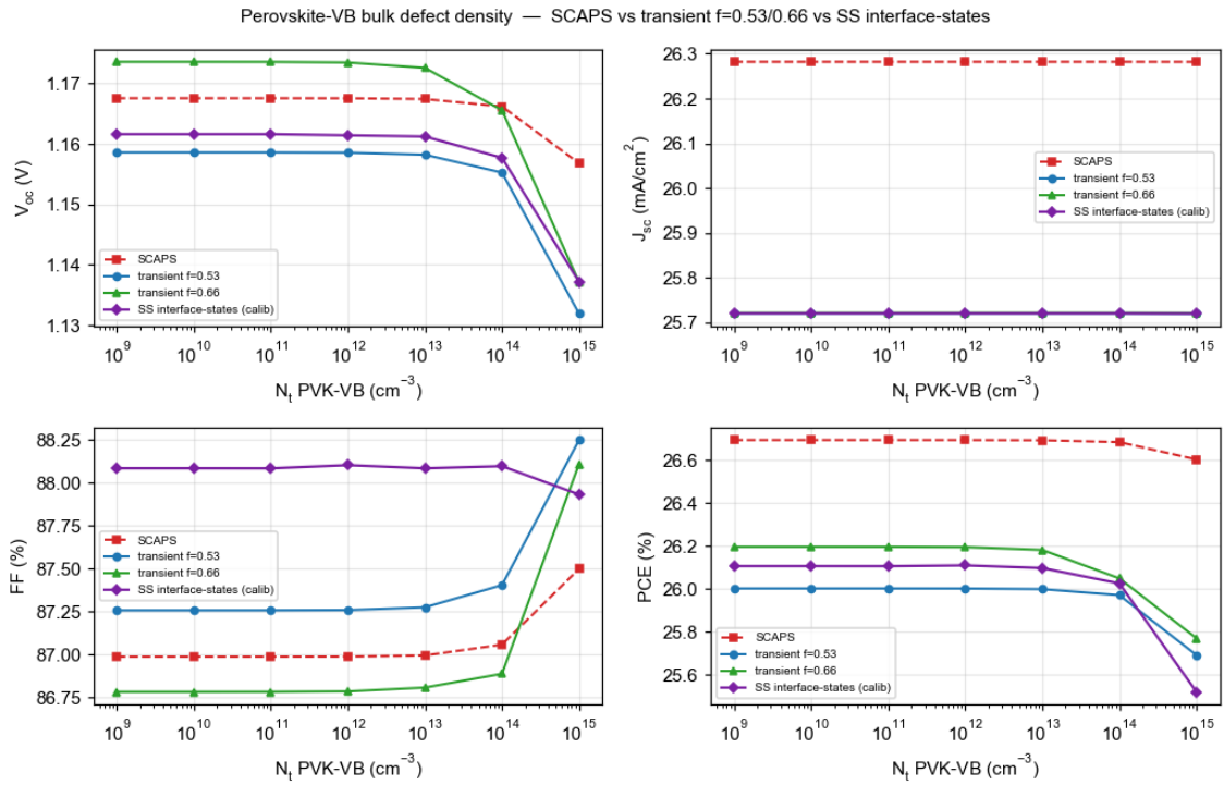
Figure 5: Perovskite-VB bulk defect density ( N_t ).
