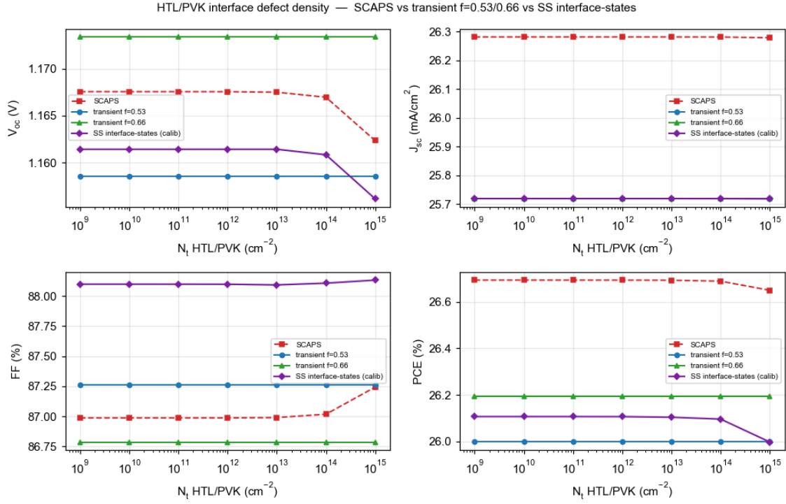
Figure 6: HTL/PVK interface defect density ( N_t ).
