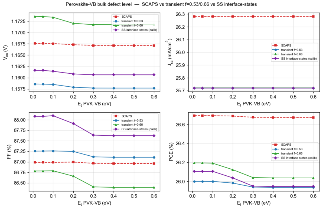
Figure 9: Perovskite-VB bulk defect level ( E_t ).
