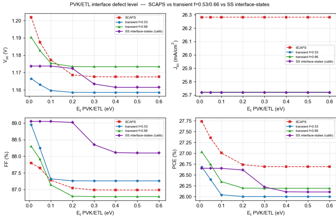
Figure 11: PVK/ETL interface defect level ( E_t ).
