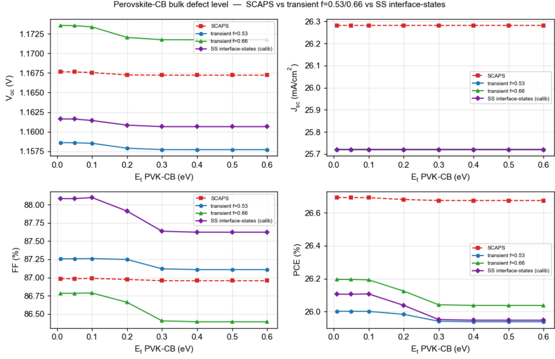
Figure 8: Perovskite-CB bulk defect level ( E_t ).
