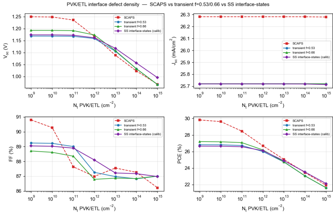
Figure 7: PVK/ETL interface defect density ( N_t ).
