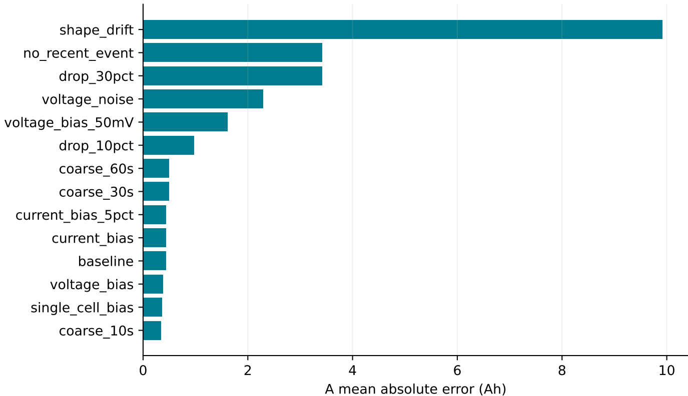
20-seed paired sensor and sampling stress; stage 2
