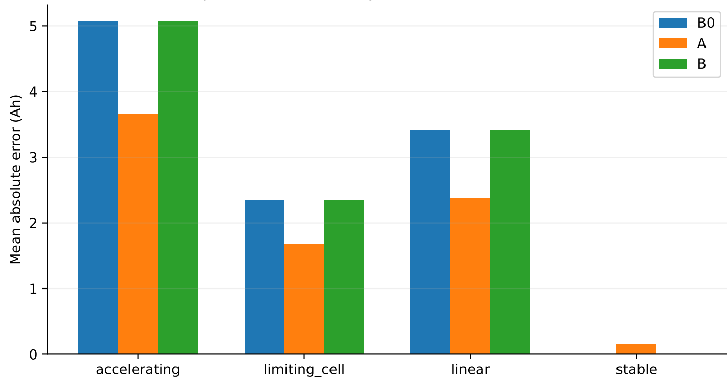
Independent two-RC + hysteresis simulator; 20 seeds
