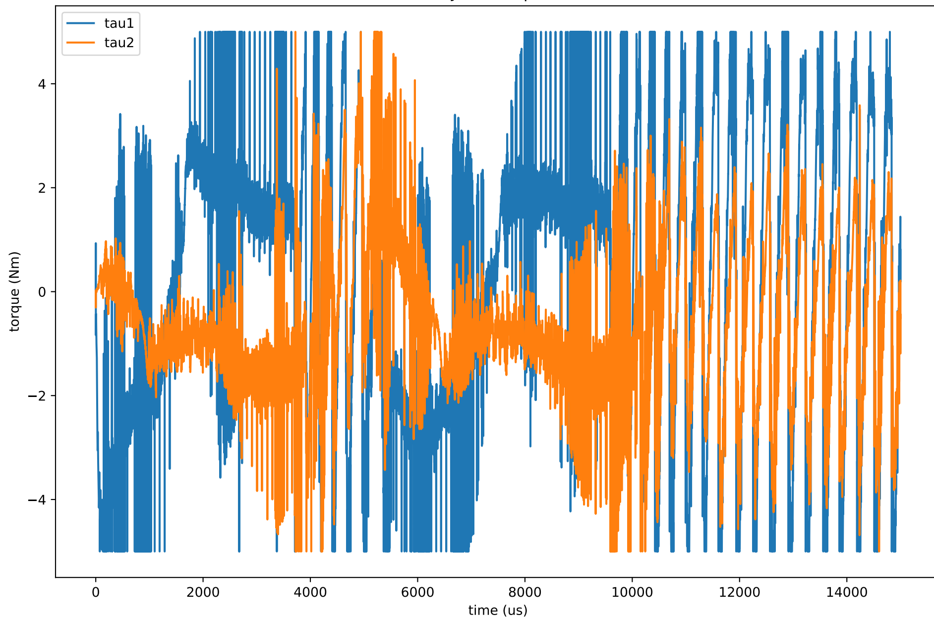
Joint Torque
