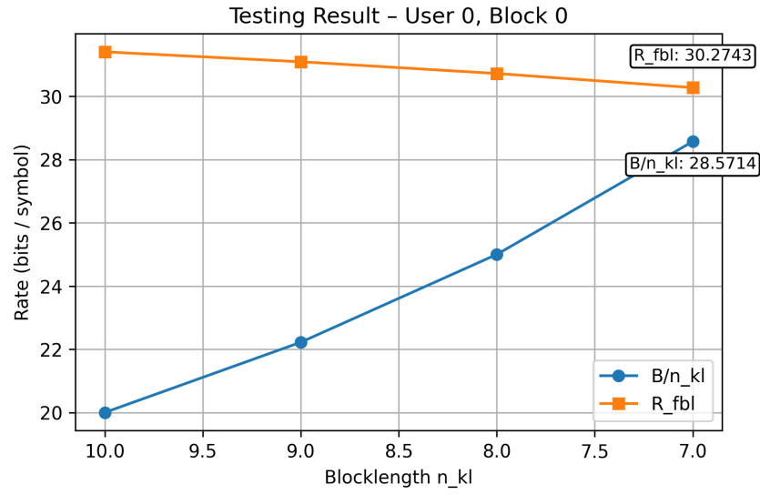
Fig. 3: Optimization performance for User 0, Block 0: Rate vs. Blocklength n_{kl} .
