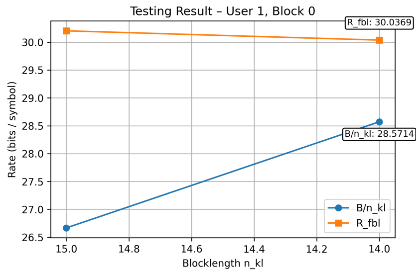
Fig. 4: Optimization performance for User 1, Block 0.
