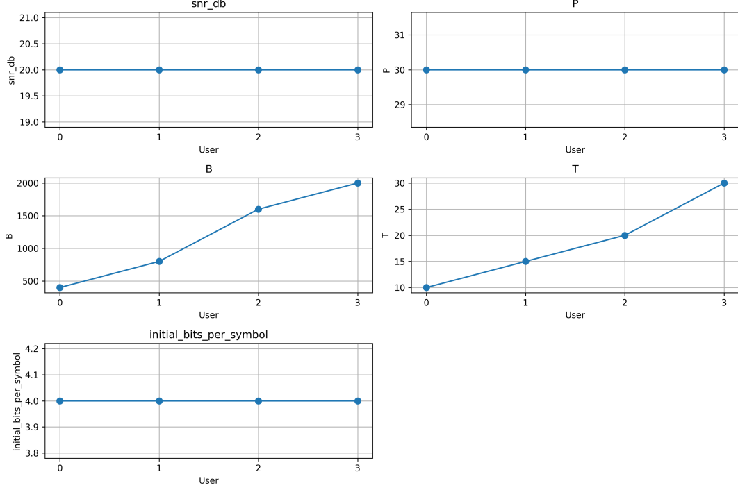
Fig. 2: Experiment configuration parameters: SNR, Power ( P ), Bandwidth ( B ), and Time ( T ) per user.
