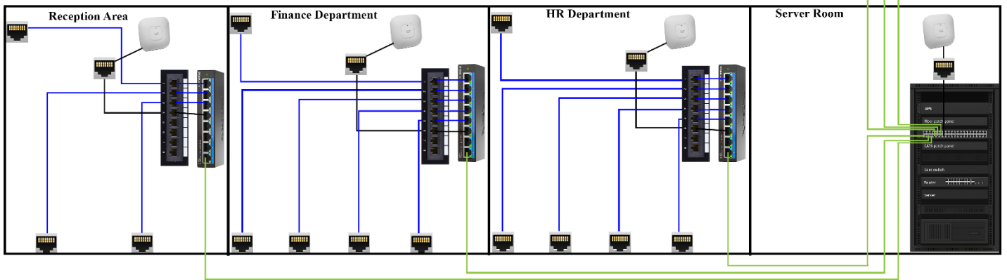
Overview of the Physical Network Design Floor plan
