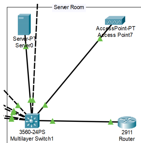
Server Room
