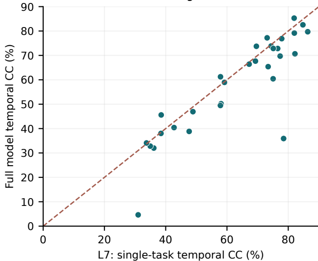
Full vs single-task
