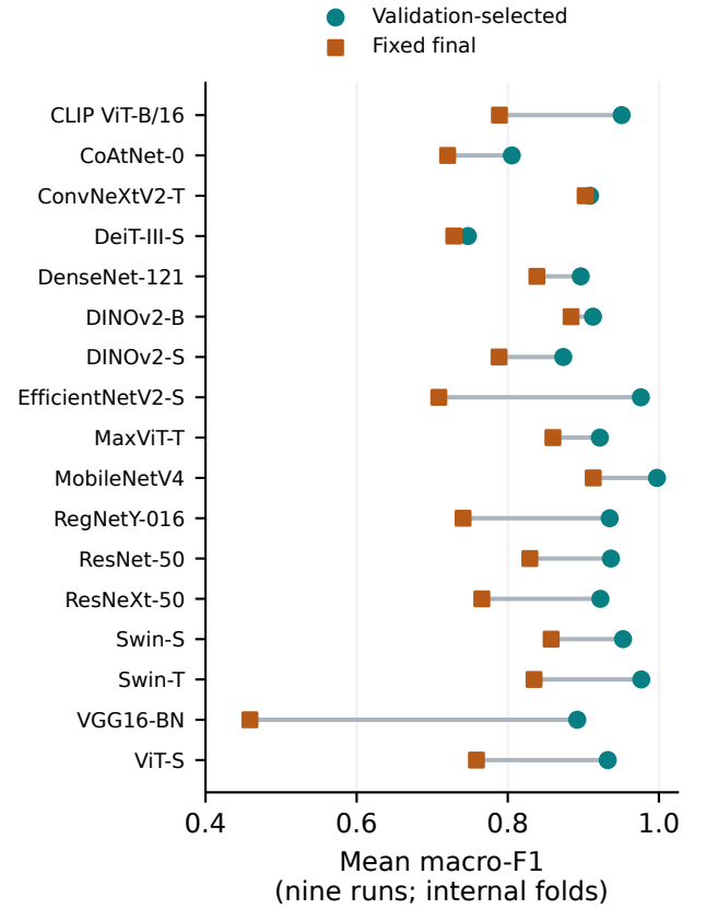
FIGURE 7. Validation-selected and fixed-final macro-F1 means for all 17 retained configurations. Each point averages nine runs on the same historical folds; connecting segments highlight endpoint differences and are not uncertainty intervals. Configurations are alphabetical, not performance-ranked.
