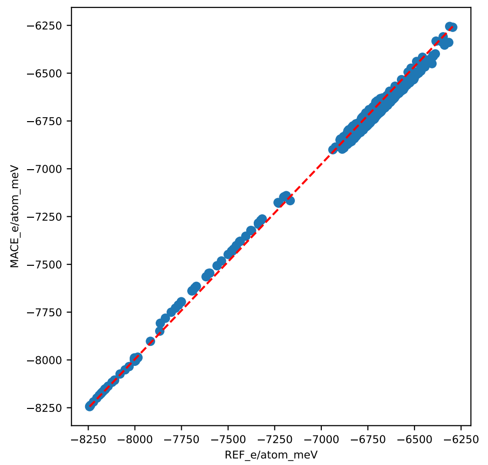
Train data
