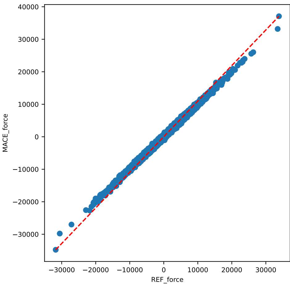
Train data
