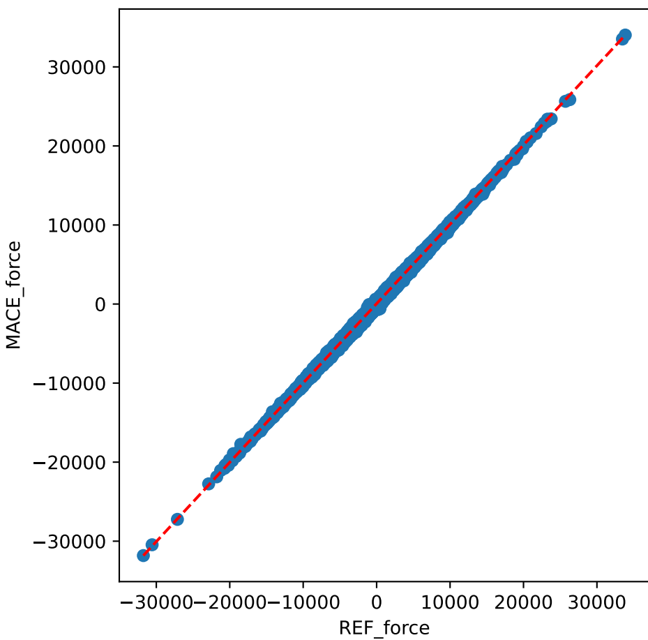
Train data
