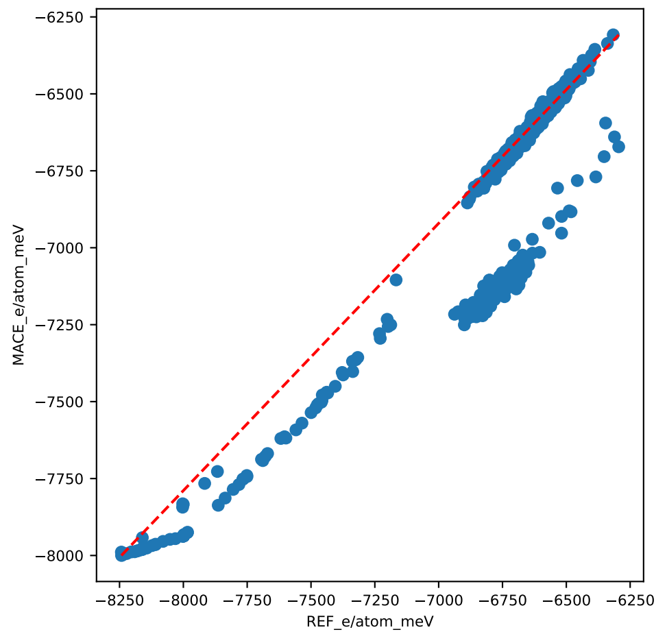
Train data
