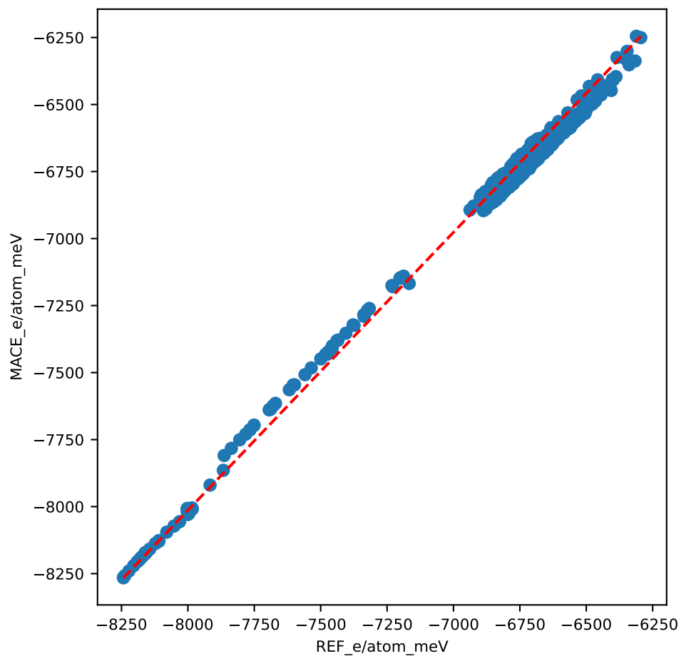
Train data
