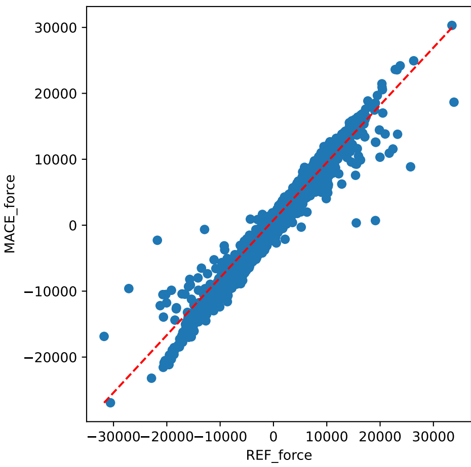
Train data
