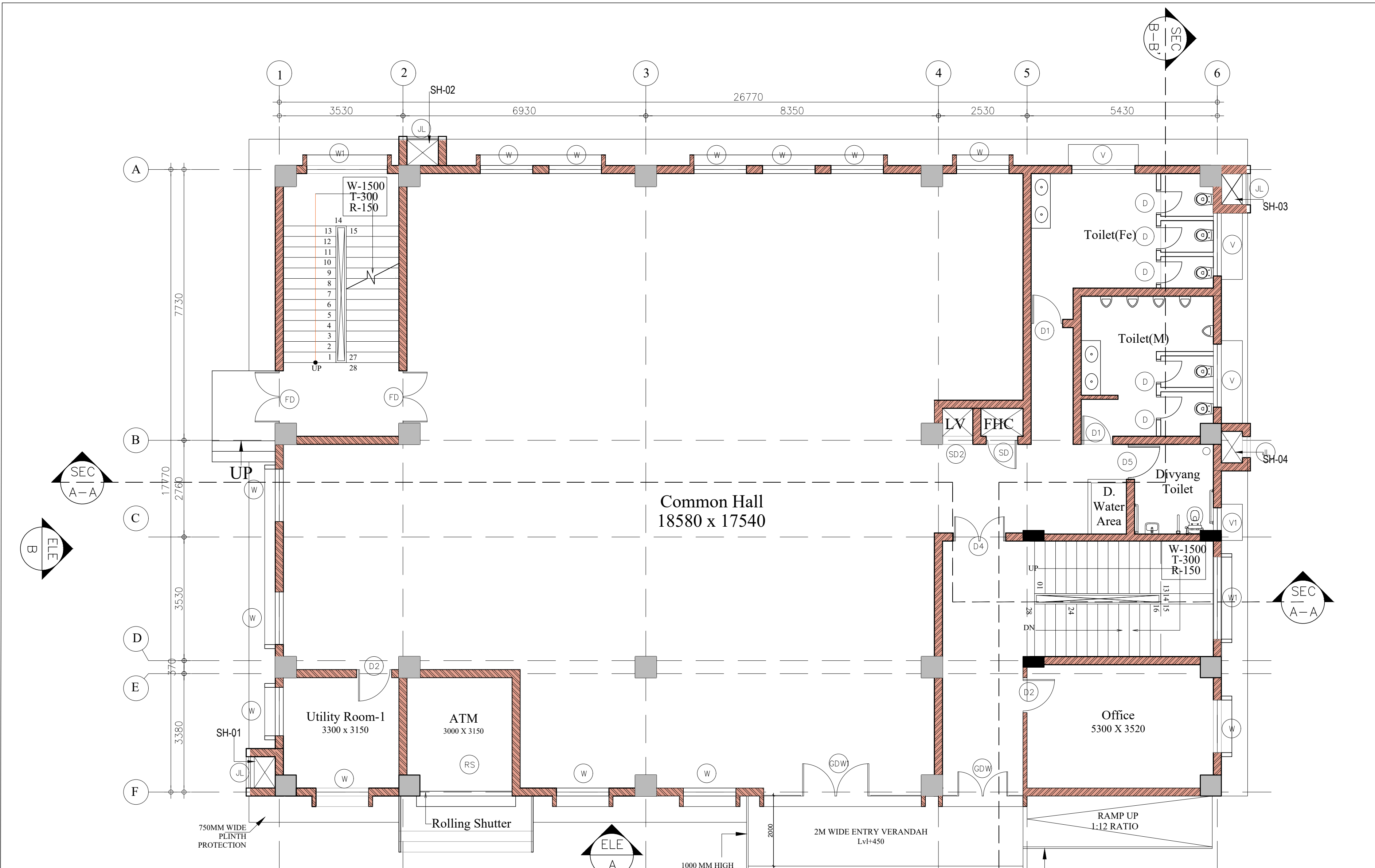
KEY PLAN
