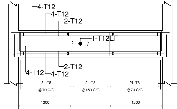
B1:300x600
