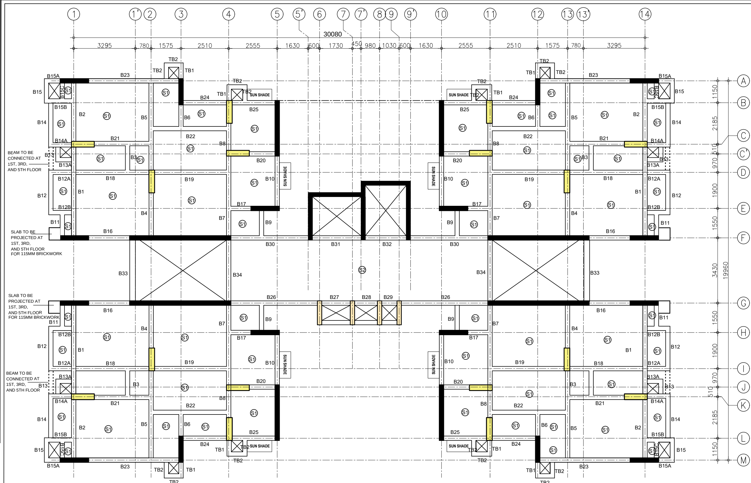
BEAM FRAMING FOR TYPICAL FLOORS
