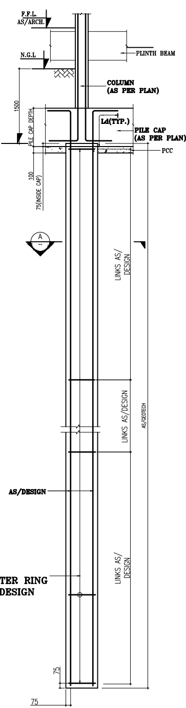
TYPICAL ELEVATION OF PILE (600MM DIA)
