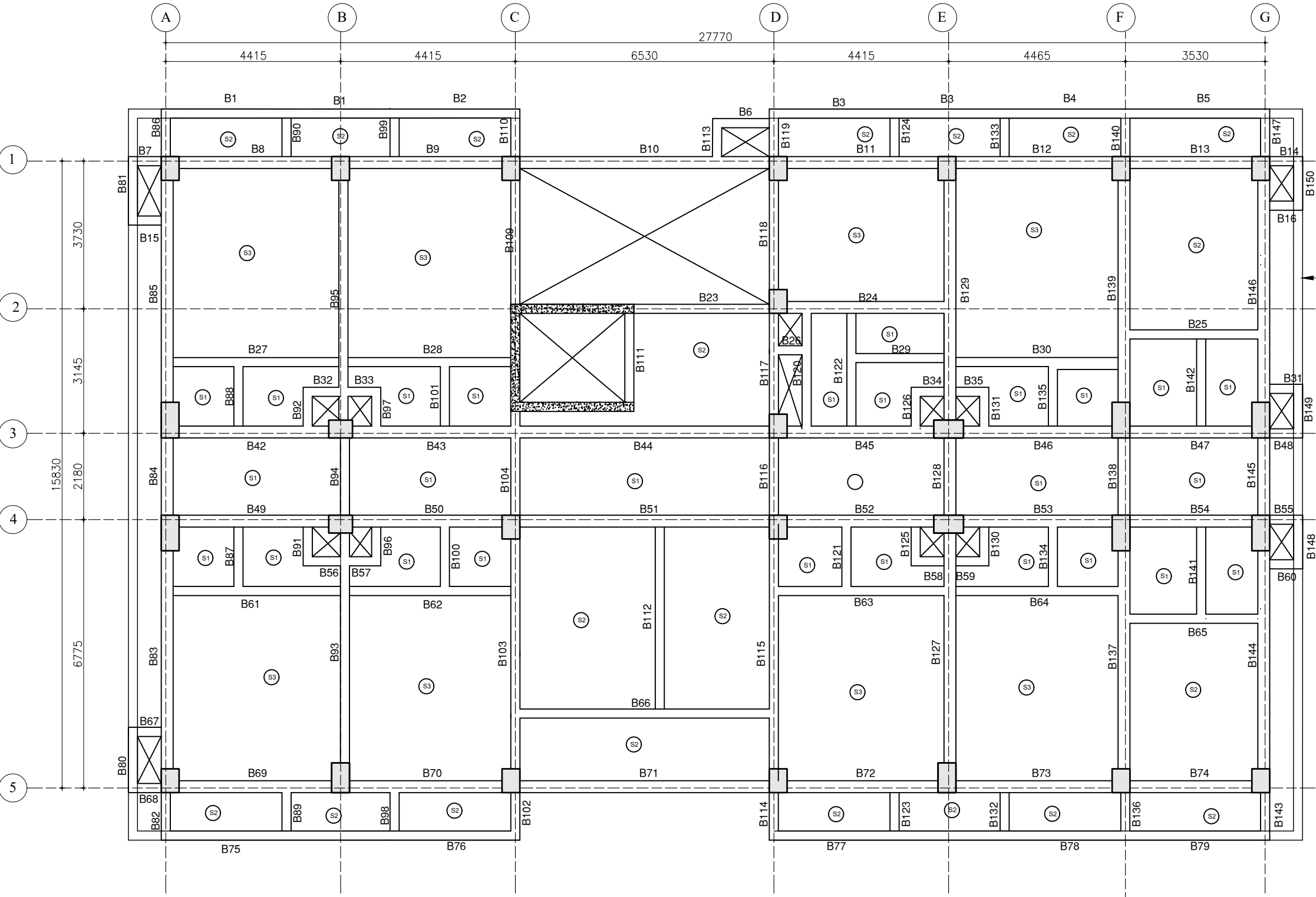
TERRACE BEAM LAYOUT PLAN
