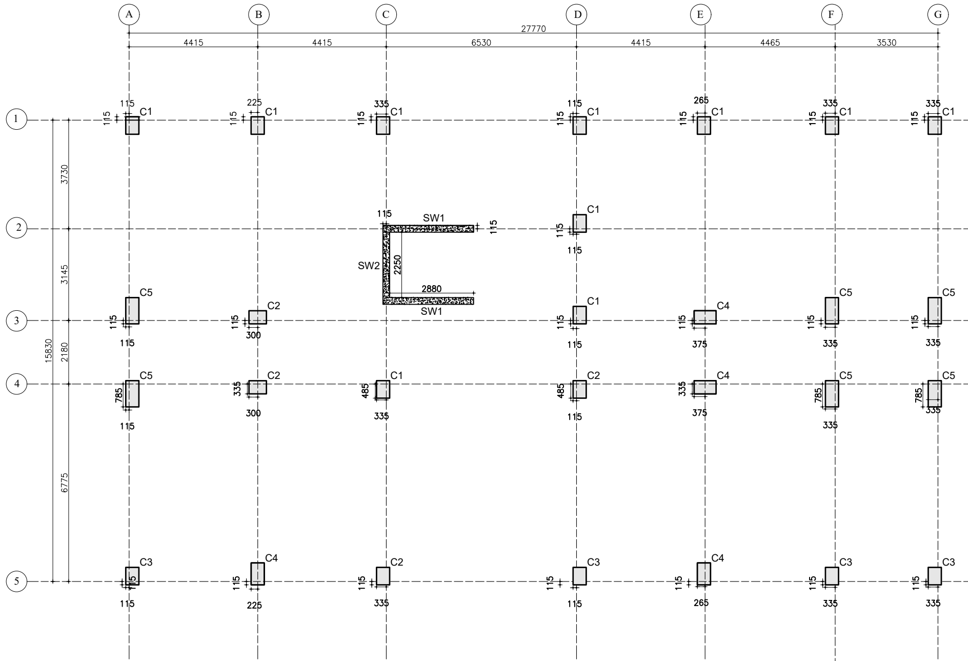
COLUMN LAYOUT PLAN
