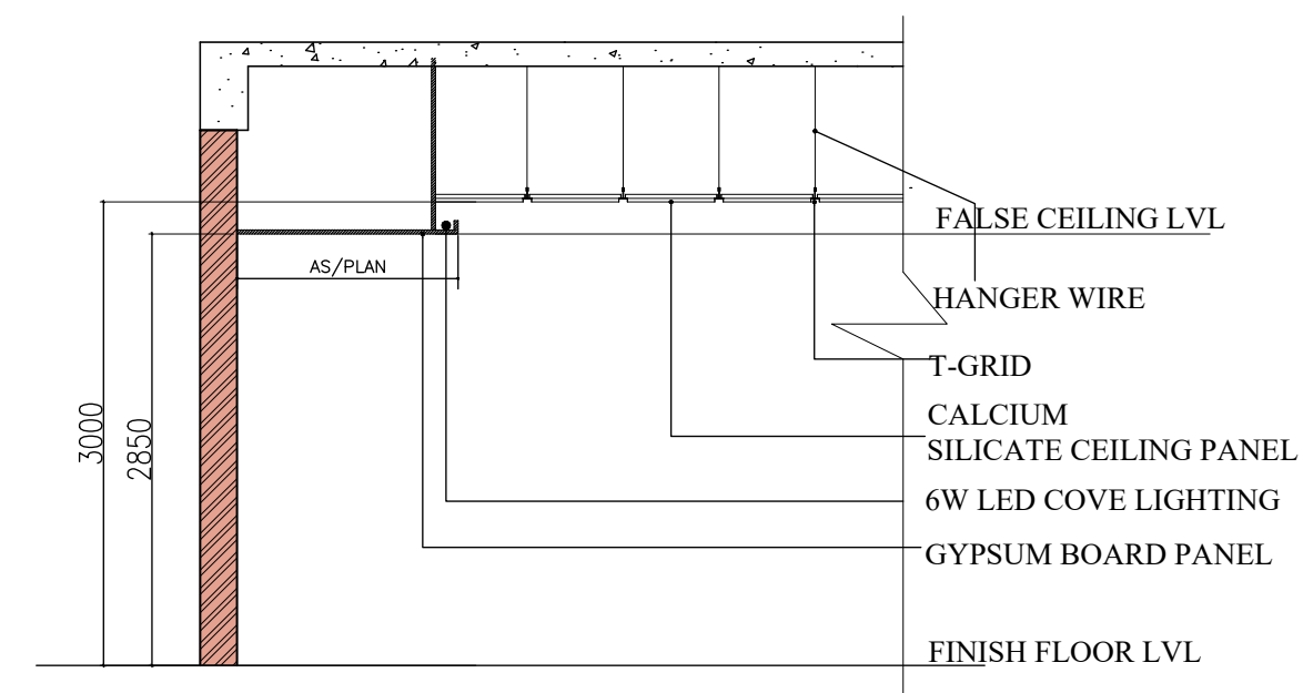
TYPICAL DETAIL-A
