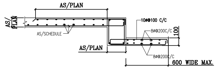
TYPICAL SUNSHADE SECTION
