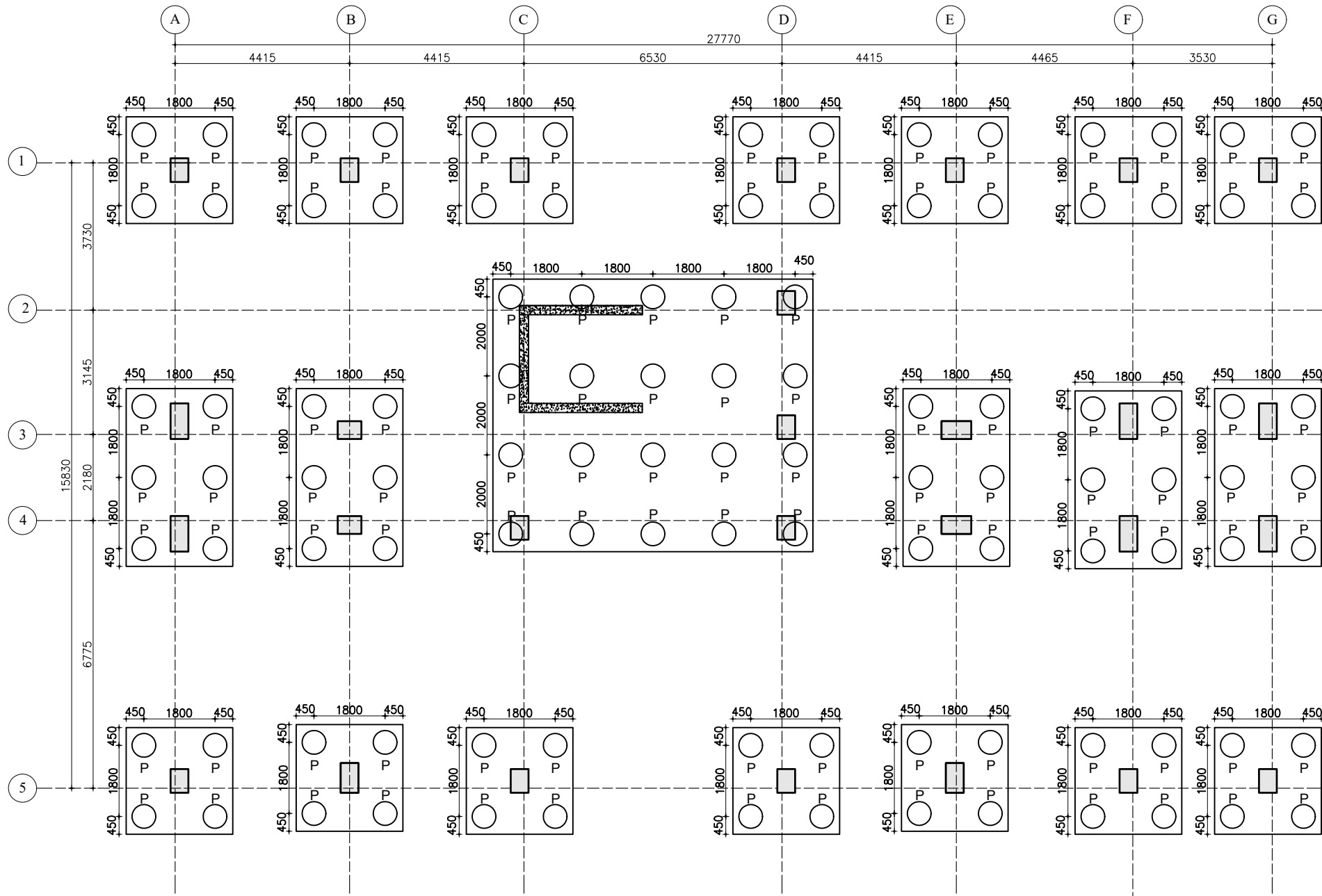
FOUNDATION LAYOUT PLAN
