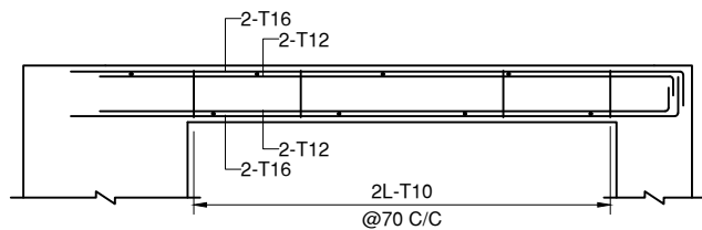
B3:230x450
