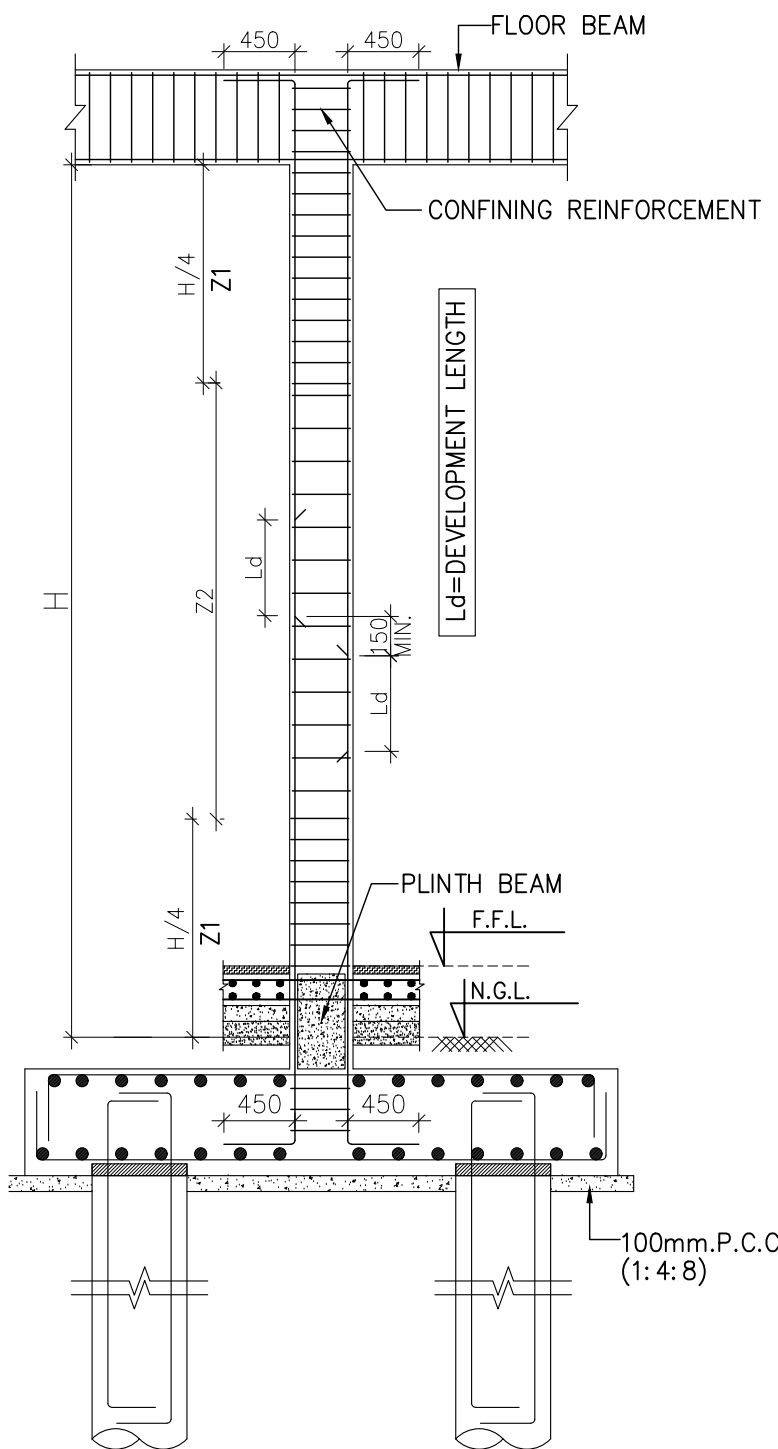
TYPICAL DETAILS FOR LAP & RING SPACING IN COLUMN DETAIL-A
