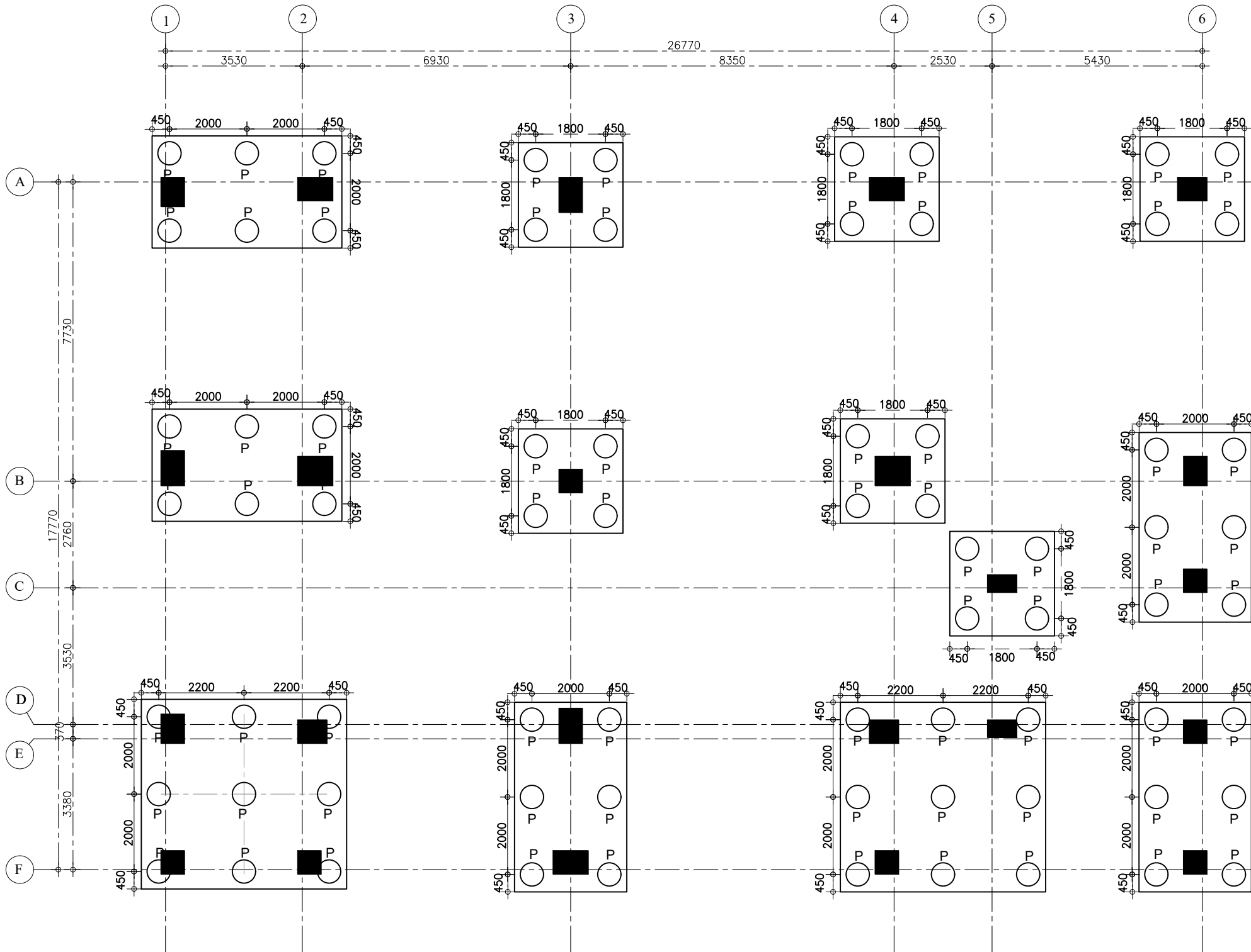
FOUNDATION LAYOUT PLAN
