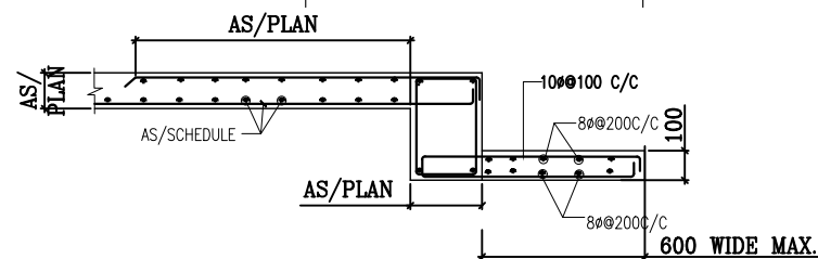
TYPICAL SUNSHADE SECTION
