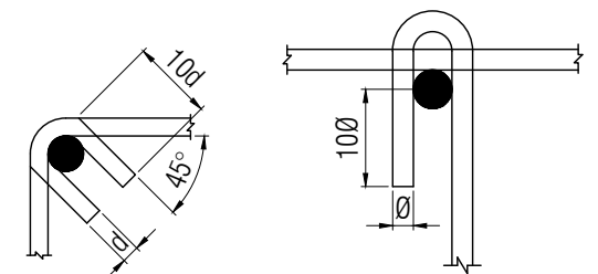
TYPICAL HOOK DETAIL
