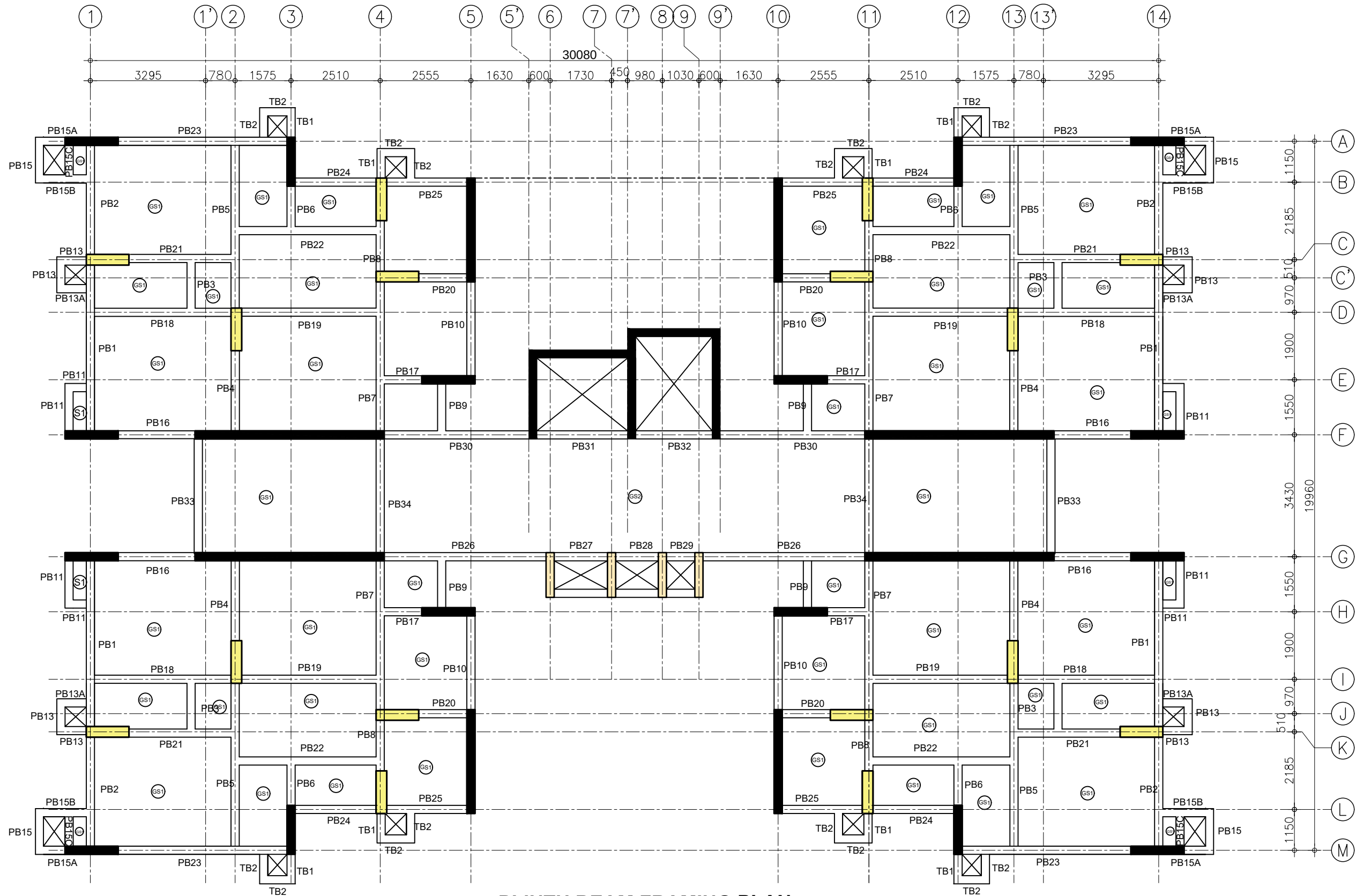
PLINTH BEAM FRAMING PLAN (ALL BEAMS AT LVL. +300MM)
