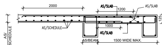
TYPICAL DETAIL FOR BALCONY
