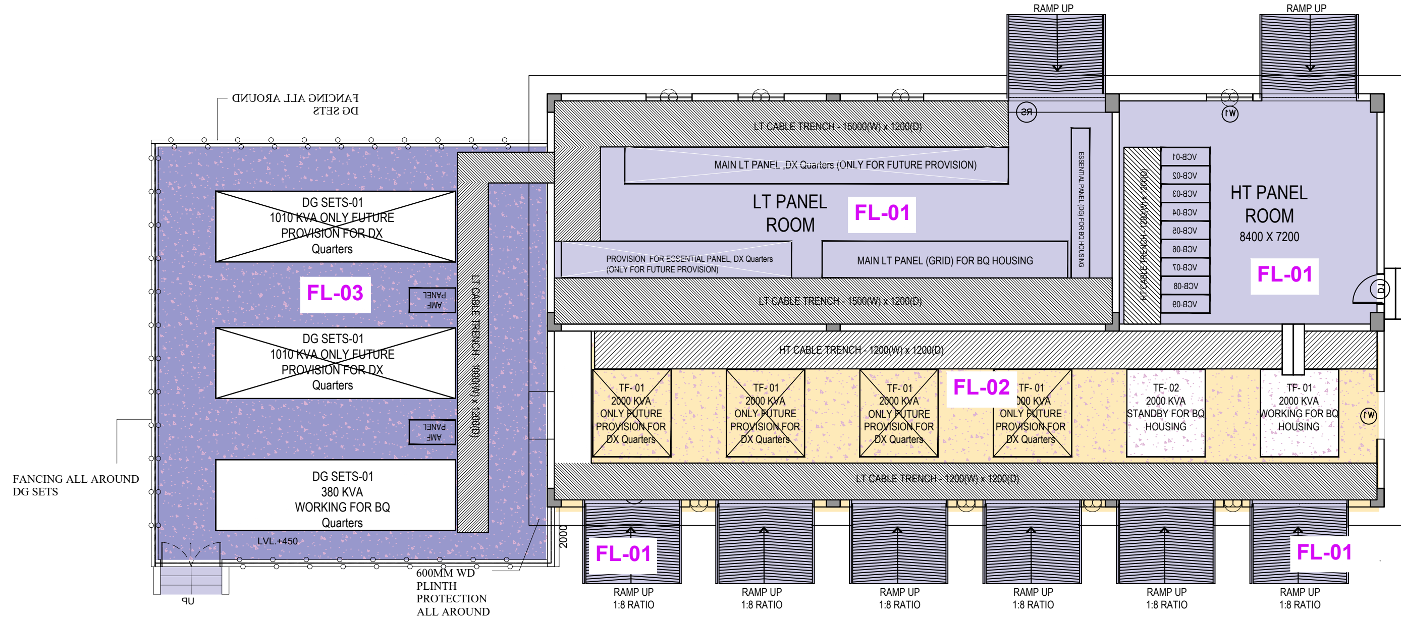
FLOOR PLAN
