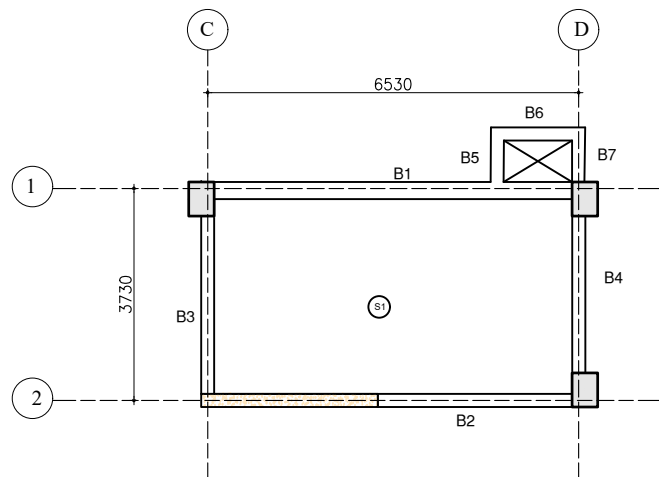
MUMTY LEVEL AND WATER TANK BOTTOM LEVEL PLAN
