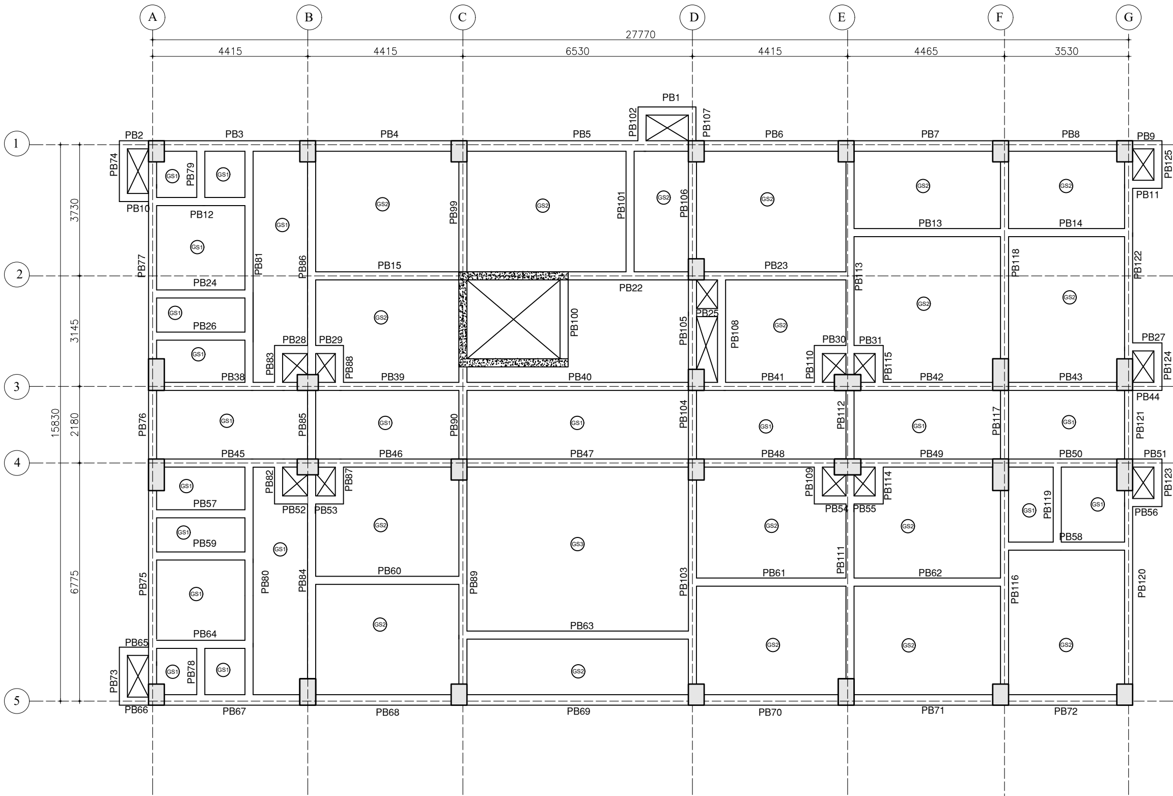
GRADE SLABS SCHEDULE DETAILS
