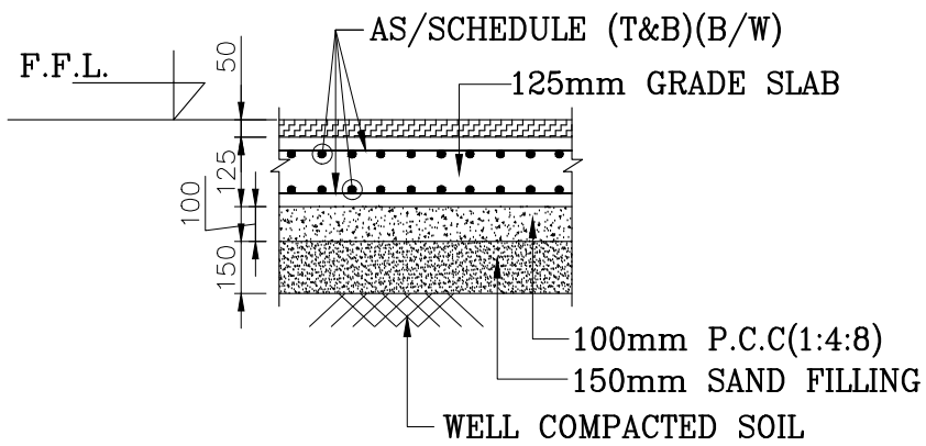
TYPICAL GRADE SLAB DETAIL
