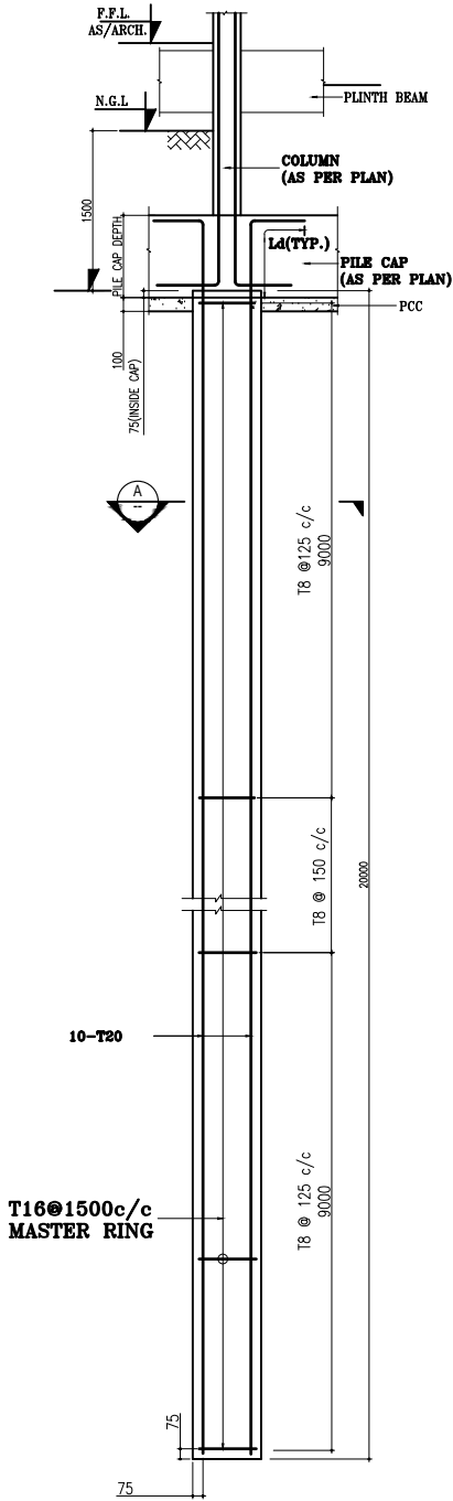
TYPICAL ELEVATION OF PILE (600MM DIA)
