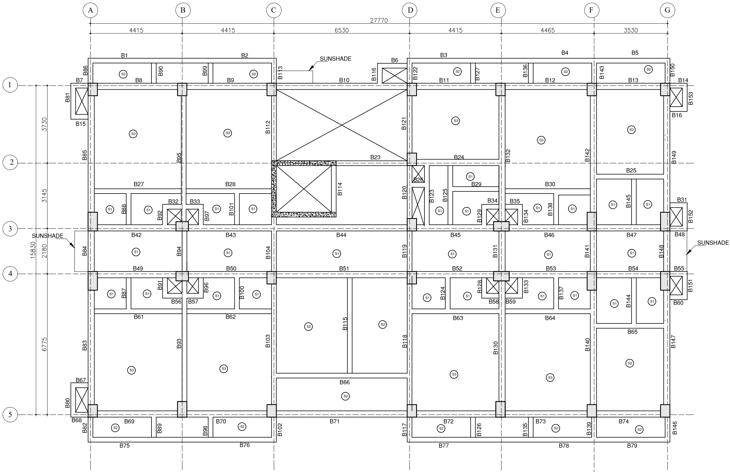
SECOND AND THIRD FLOOR BEAM LAYOUT PLAN
