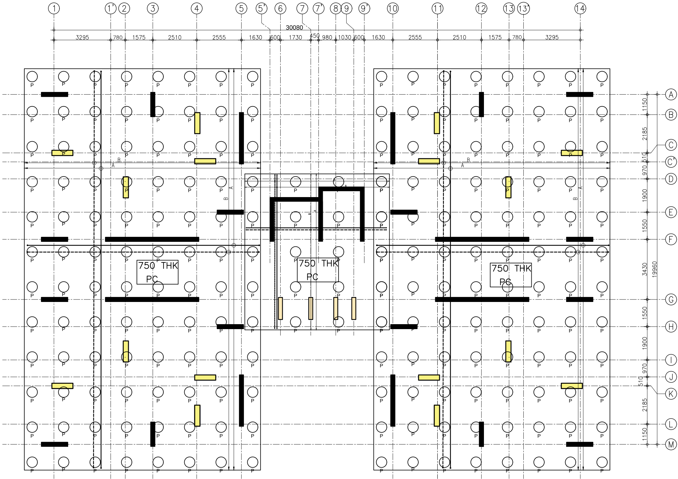
PILE CAP LAYOUT PLAN
