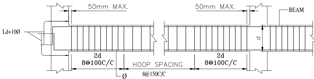
TYPICAL BEAM SHEAR R/F DETAIL
