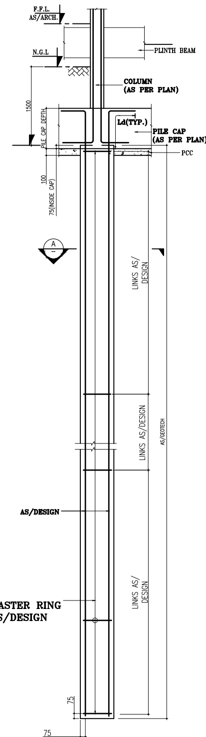
TYPICAL ELEVATION OF PILE (600MM DIA)
