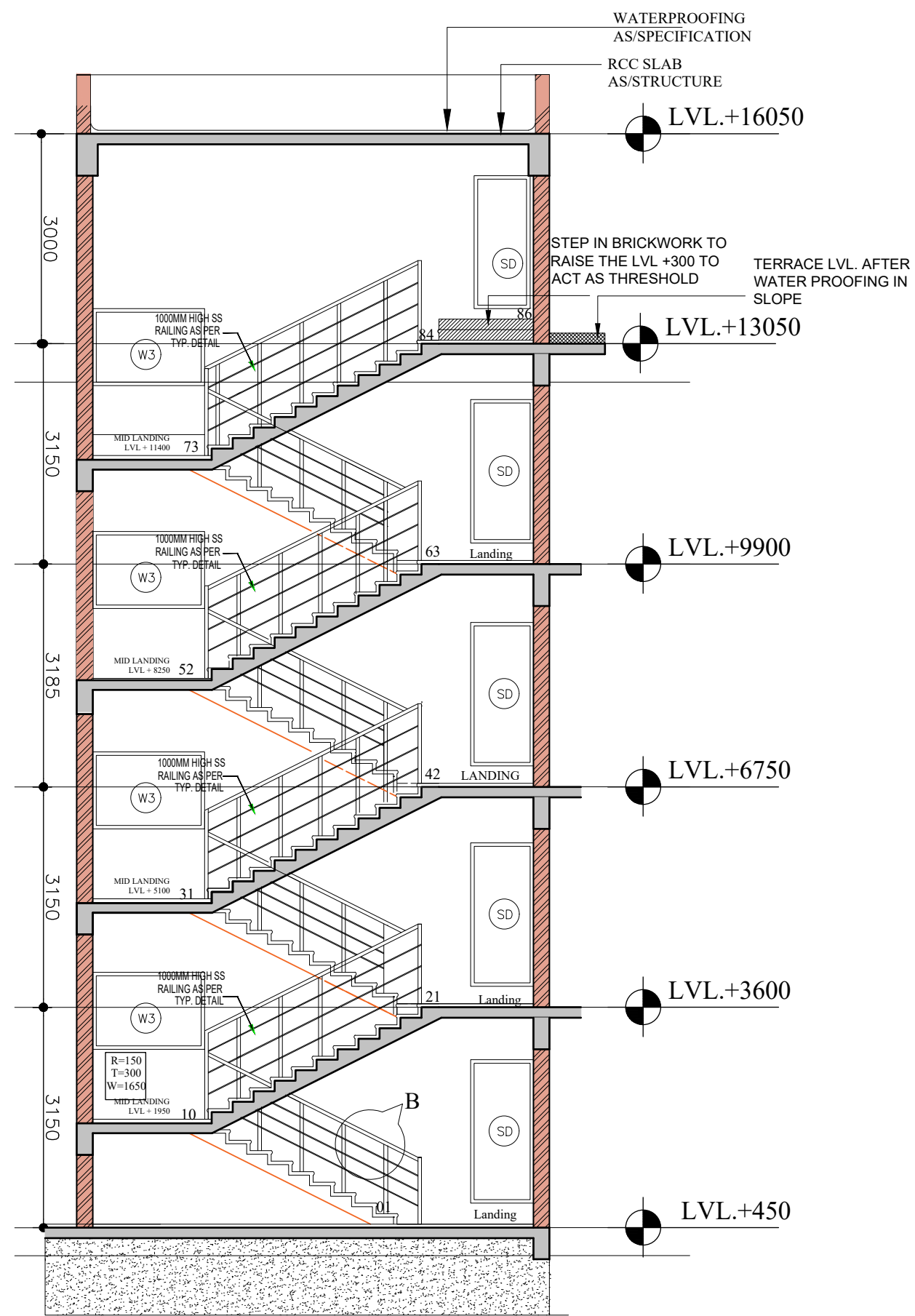
SECTION YY
