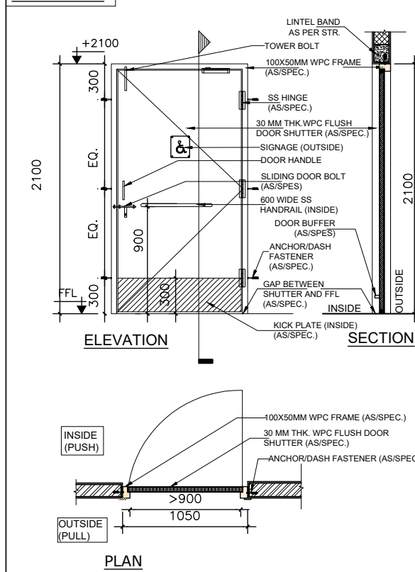
DOOR-D3
