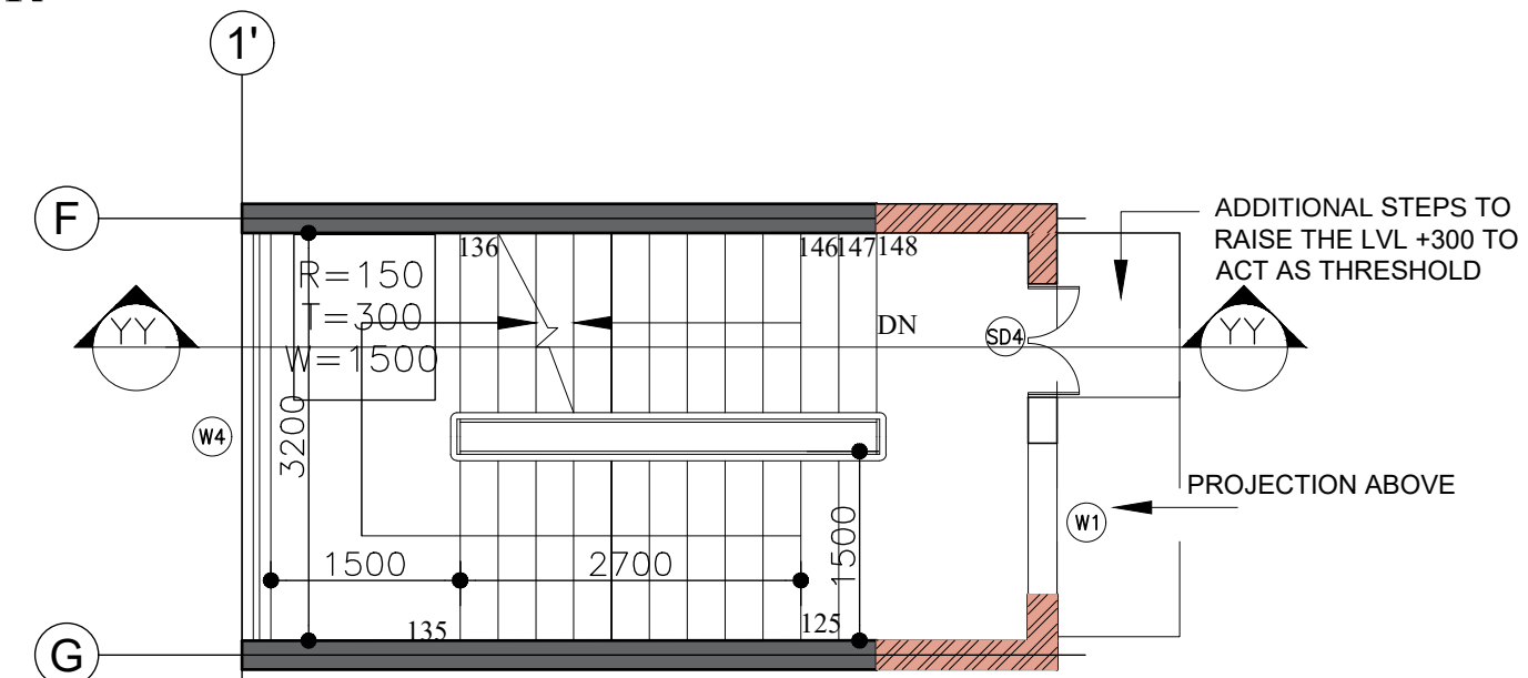
STAIRCASE PLAN AT TYPICAL FLOOR
