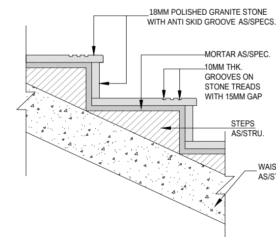
STEPS DETAIL
