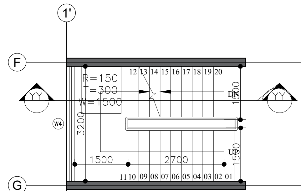
TYPICAL STAIRCASE PLAN AT GROUND FLOOR
