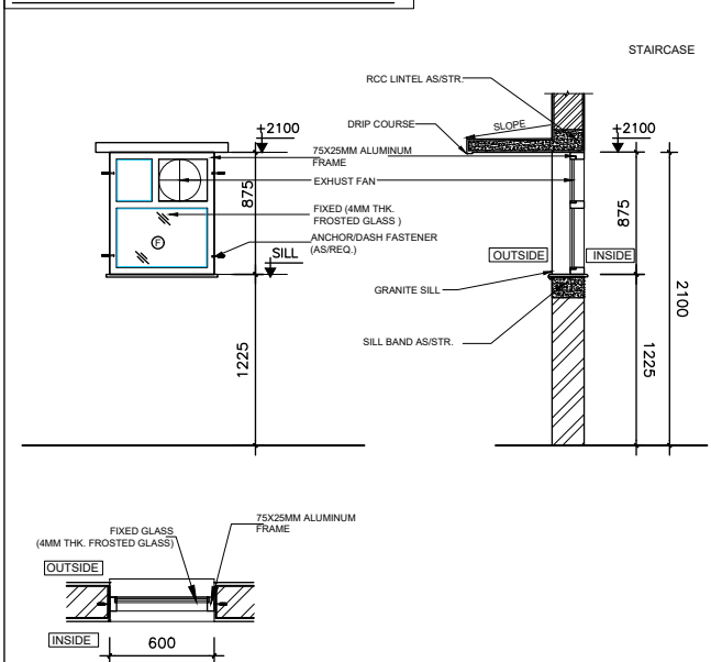
TYPICAL TOILET VENTILATOR -V
