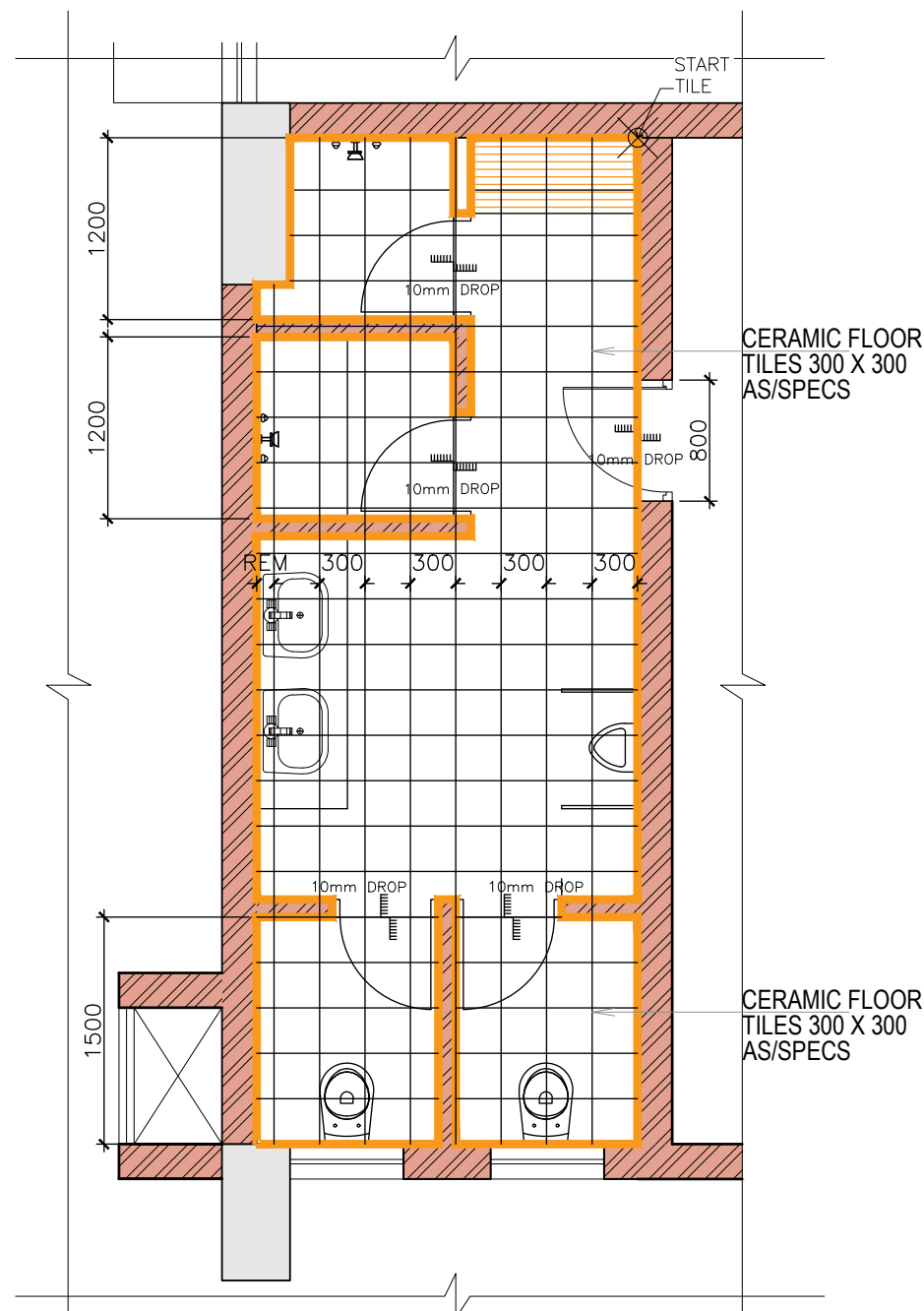
02 PLAN_FLOORING
