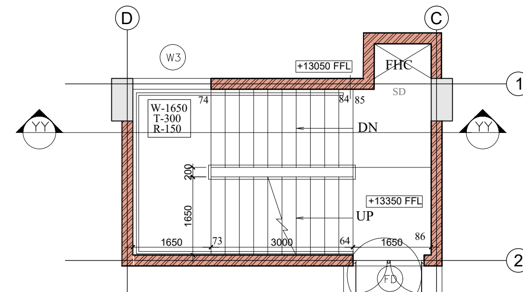
TYPICAL STAIRCASE PLAN AT THIRD FLOOR
