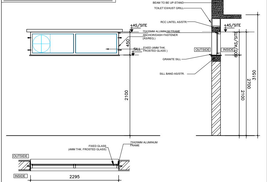
TYPICAL TOILET VENTILATOR -V1
