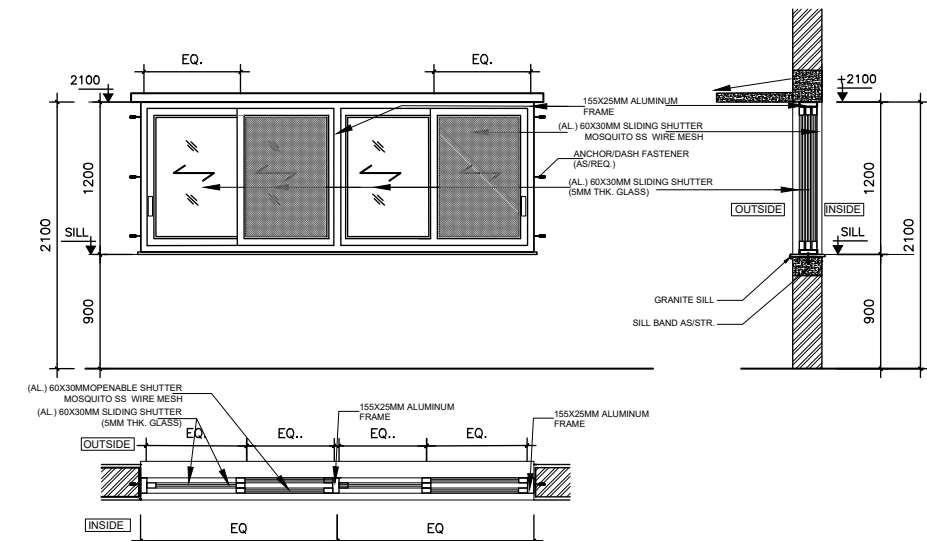
TYPICAL WINDOW -W1
