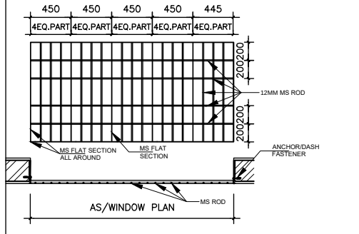
TYPICAL MS GRILL ALL AROUND WINDOW OPENING
