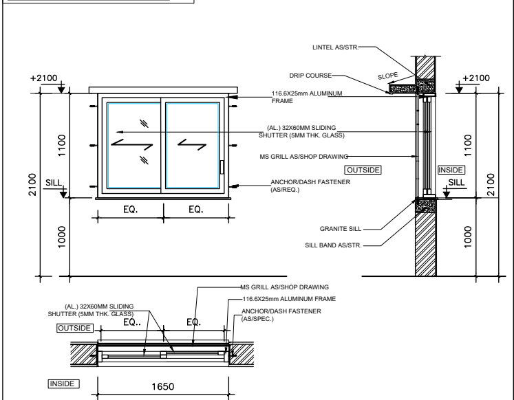
TYPICAL WINDOW -W3
