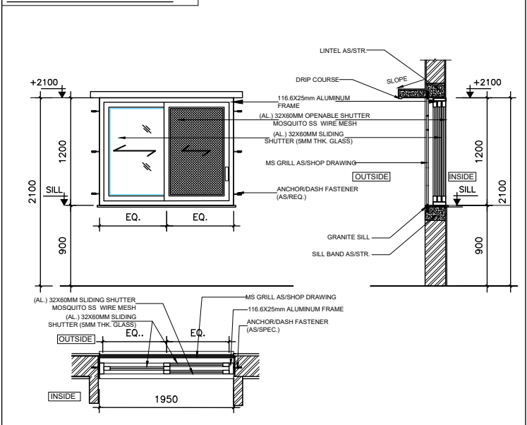
TYPICAL WINDOW -W4
