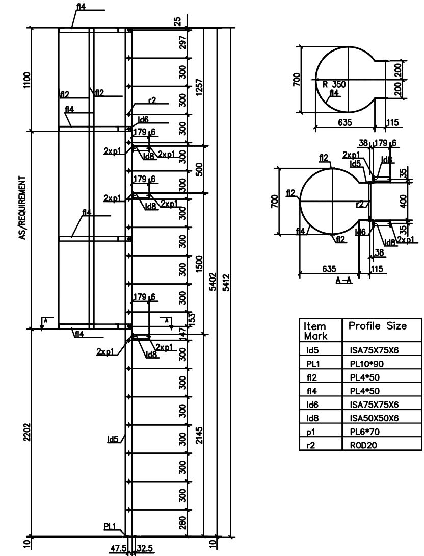
STAIRCASE RAILING DETAIL DETAIL B
