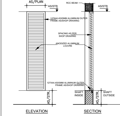
JL-TYPICAL ALUMINUM FRAME- OPENABLE LOUVERED PANEL
