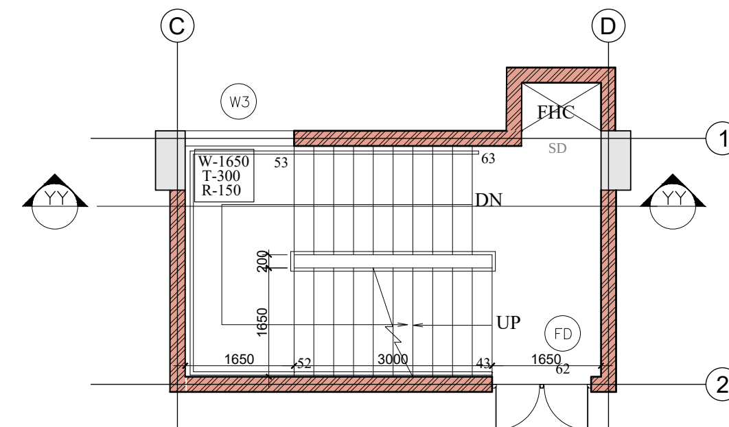
TYPICAL STAIRCASE PLAN AT SECOND FLOOR
