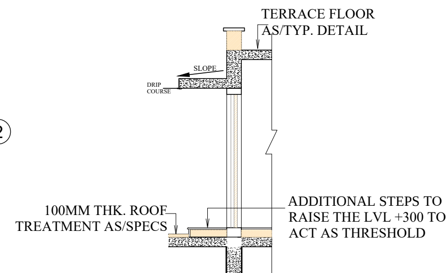
DETAIL D
