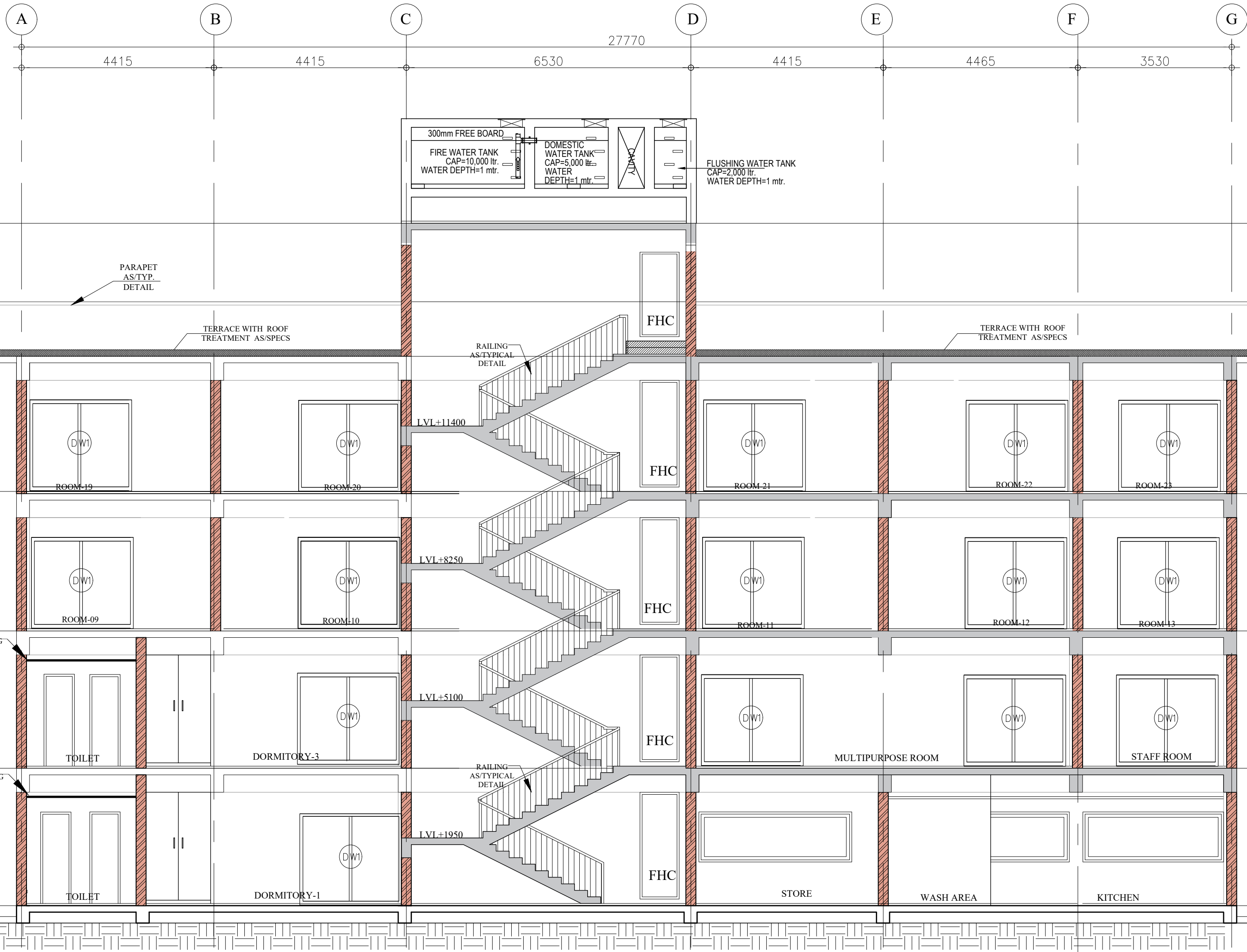
SECTION-AA
