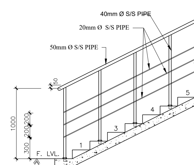
STAIRCASE RAILING DETAIL
