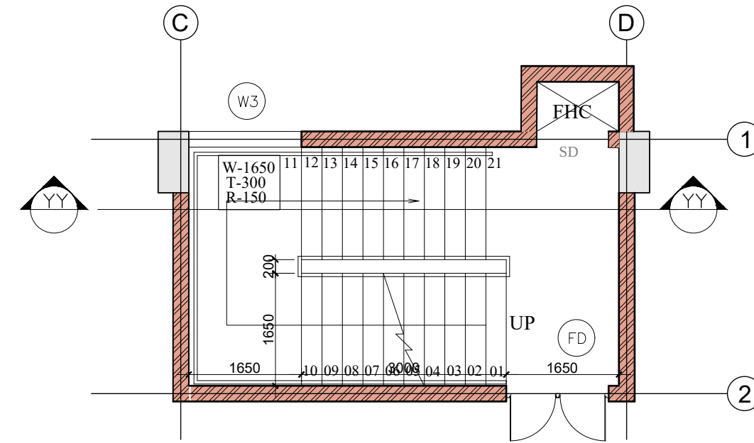
TYPICAL STAIRCASE PLAN AT GROUND FLOOR
