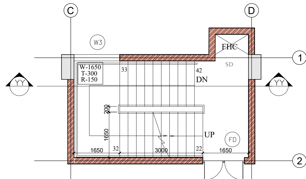
TYPICAL STAIRCASE PLAN AT FIRST FLOOR
