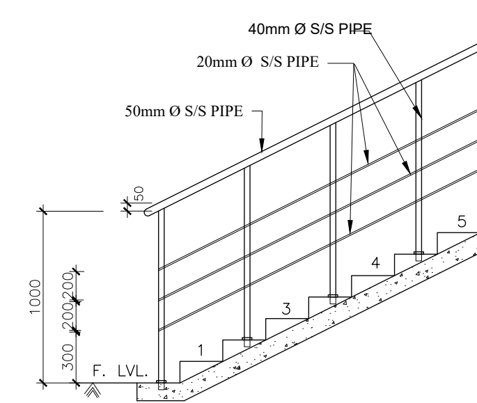
STAIRCASE RAILING DETAIL DETAIL B
