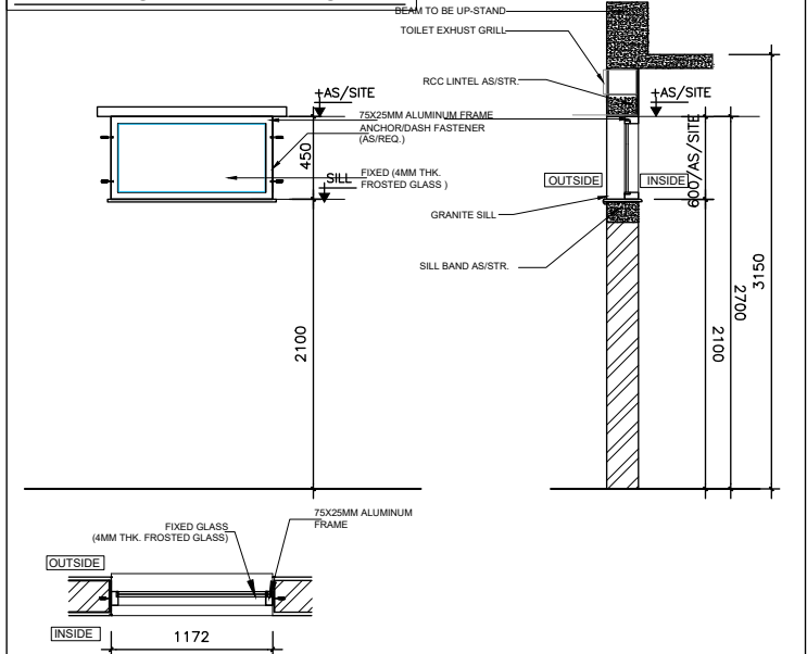
TYPICAL TOILET VENTILATOR -V2
