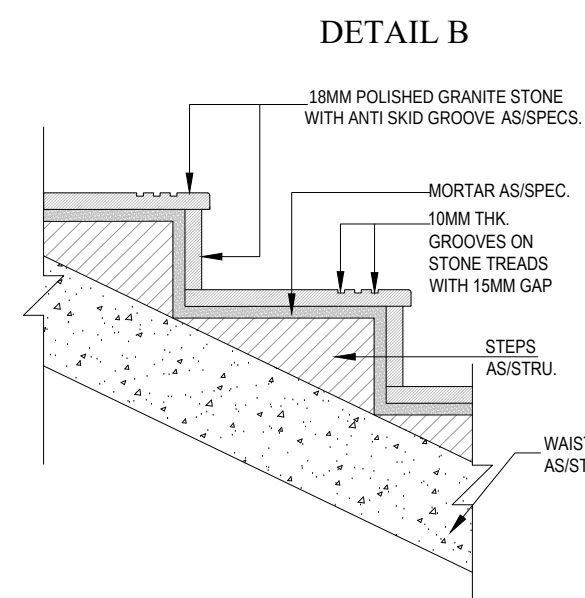
STAIRCASE DETAIL
