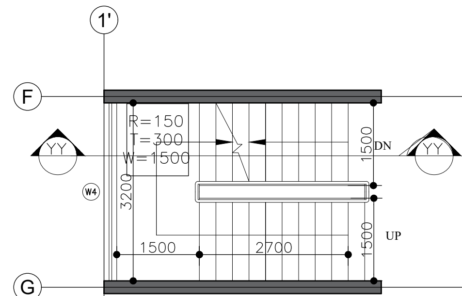
STAIRCASE PLAN AT TYPICAL FLOOR
