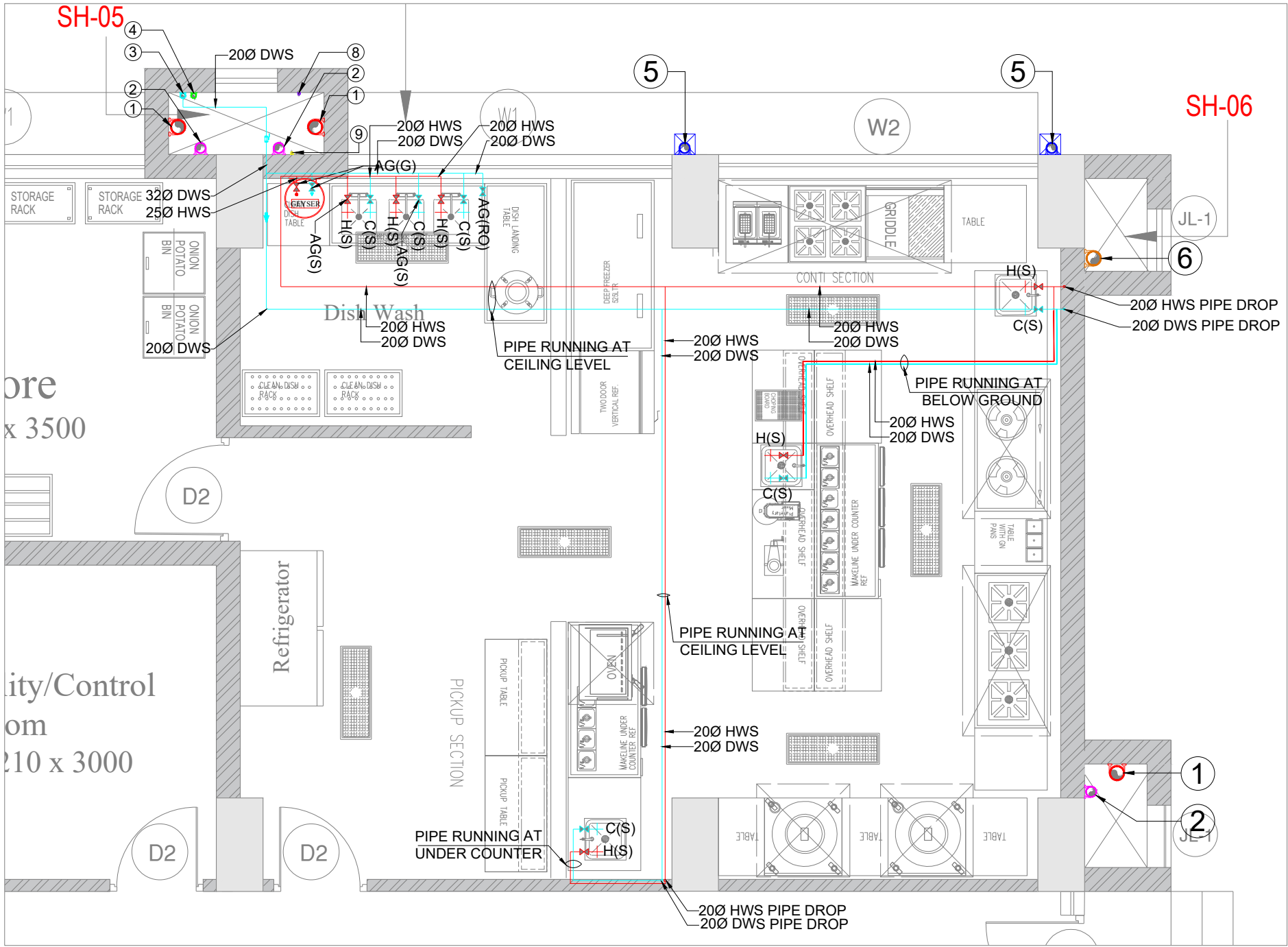
KITCHEN WATER SUPPLY LAYOUT
