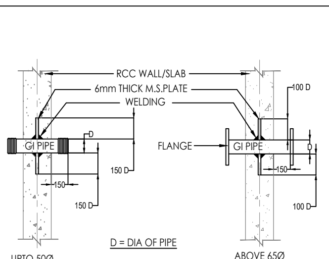
PUDDLE FLANGE DETAIL
