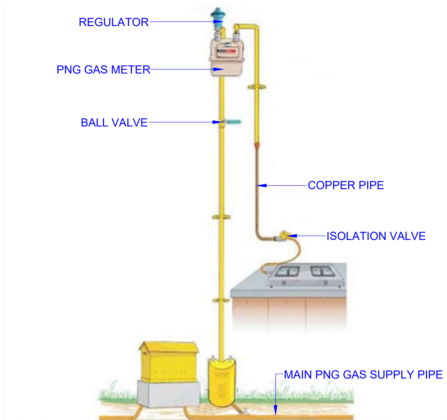
DOMESTIC GAS CONNECTION SCHEMATIC
