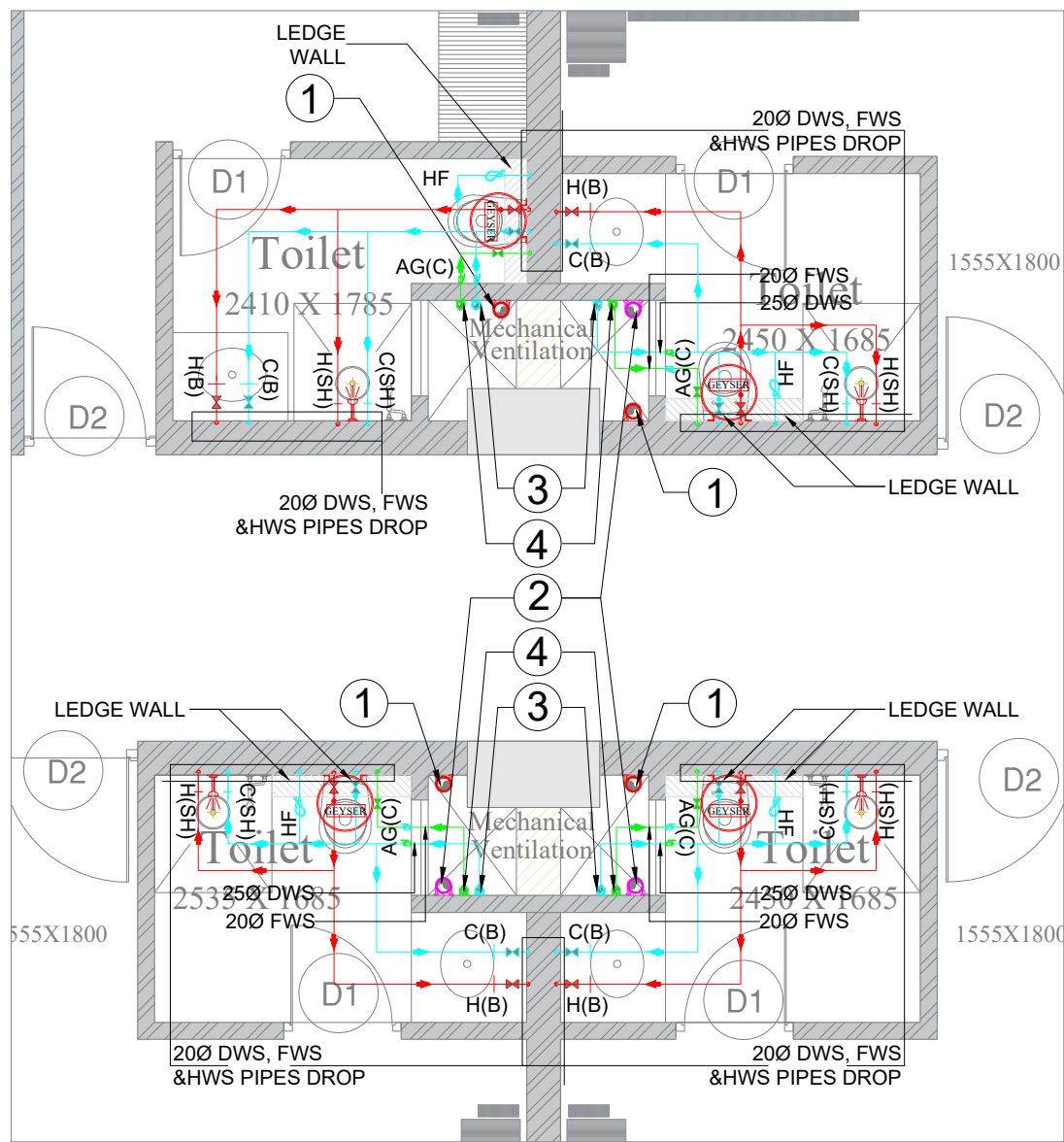
TYPICAL TOILET WATER SUPPLY LAYOUT
