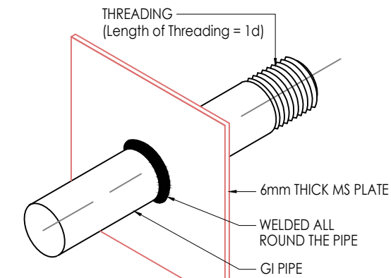
ISOMETRIC PUDDLE FLANGEDETAIL
