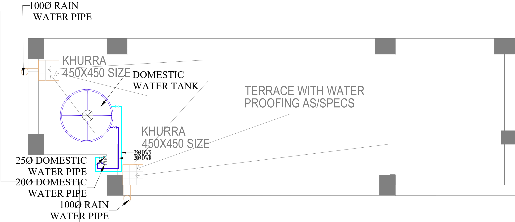
TERRACE PLAN PLUMBING LAYOUT
