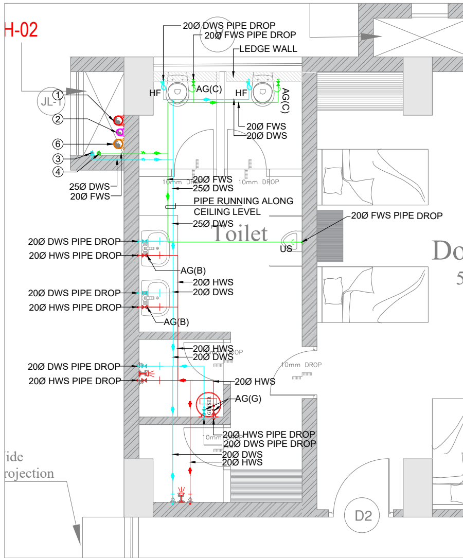
TYPICAL TOILET WATER SUPPLY LAYOUT
