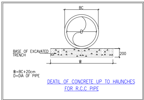
HAUNCHING DETAIL SCALE=NTS
