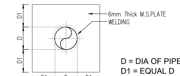
PUDDLE FLANGE DETAIL (PIPE SIZE ABOVE 80mm DIA)
