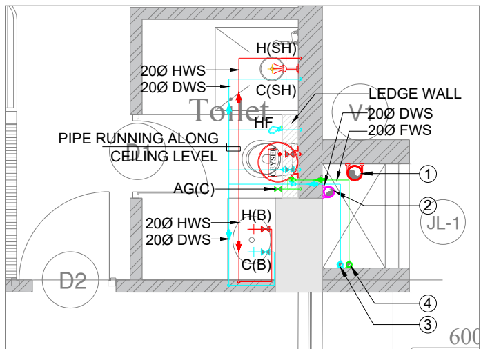
TYPICAL TOILET WATER SUPPLY LAYOUT
