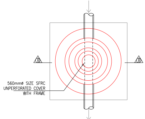
CIRCULAR MANHOLE 1220 DIA FOR SEWERAGE SYSTEM WITH TYPE-B - DEPTH 1.651m TO 2.300m
