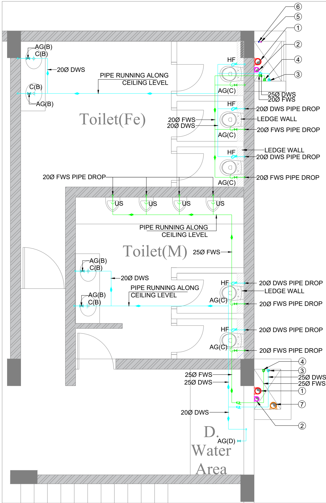
1st FLOOR TOILET WATER SUPPLY LAYOUT
