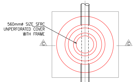
CIRCULAR MANHOLE 910 DIA FOR SEWERAGE SYSTEM TYPE-A - DEPTH 0.901m TO 1.650m
