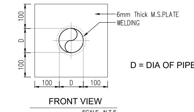
PUDDLE FLANGE DETAIL (PIPE SIZE UP TO 80mm DIA)
