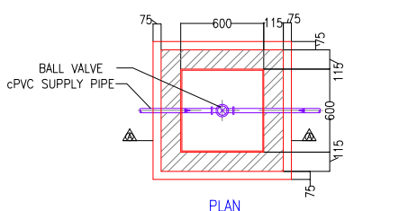
TYPICAL DETAIL OF VALVE WITH CHAMBER
