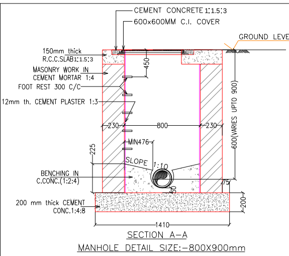
SECTION A-A MANHOLE DETAIL SIZE:-800X900mm
