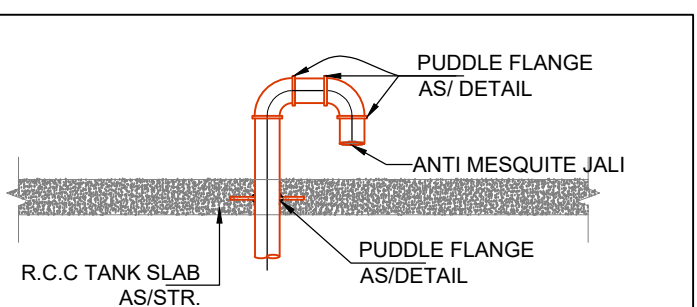
TYPICAL VENT PIPE DETAIL SCALE=NTS
