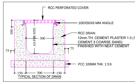
RCC DRAIN SECTION
