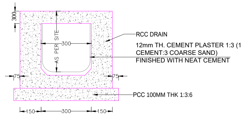
RCC DRAIN SECTION AT ROAD CROSSING
