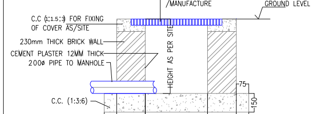
SECTION A-A TYPICAL DETAIL OF CATCH BASIN
