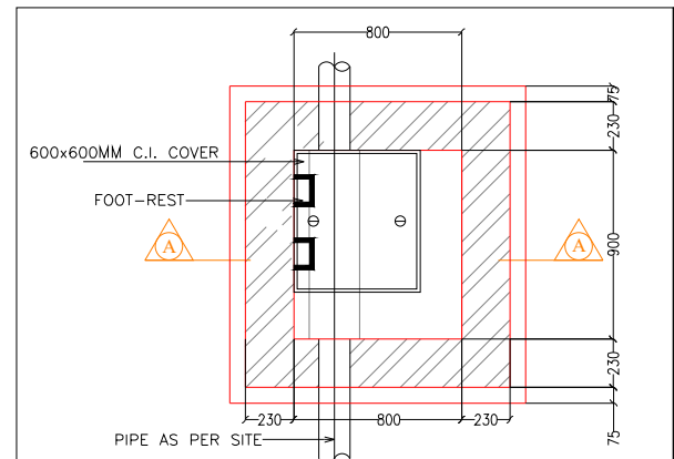
PLAN RECTANGULAR MANHOLE 800X900mm FOR SEWERAGE SYSTEM TYPE-a DEPTH 600 TO 900mm
