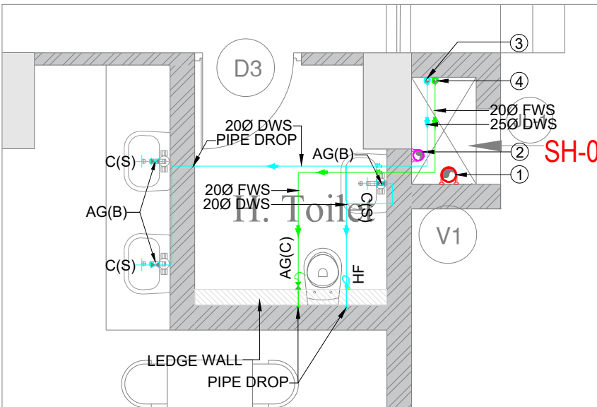
HANDICAP TOILET WATER SUPPLY LAYOUT
