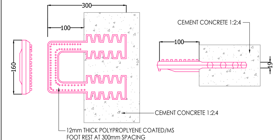
TYPICAL FOOT REST DETAIL
