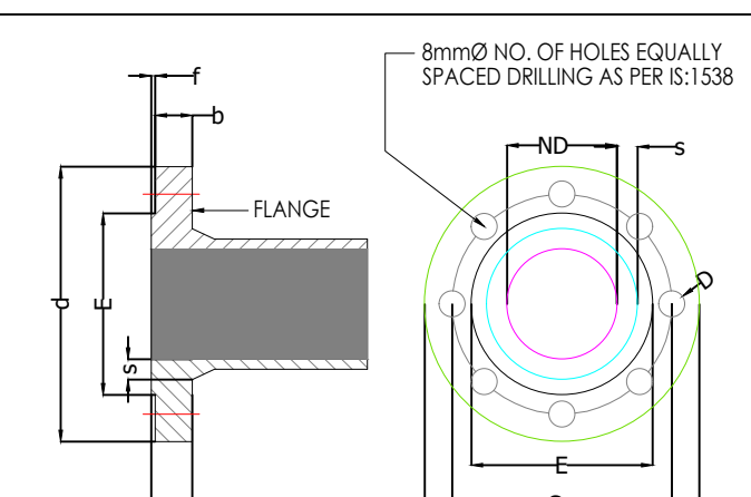
(FLANGE) DETAIL-C
