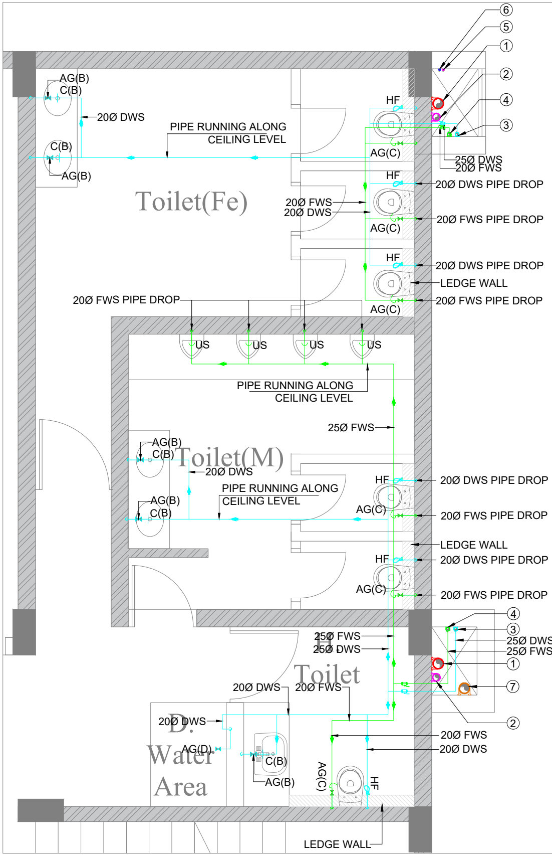
GROUND FLOOR TOILET WATER SUPPLY LAYOUT
