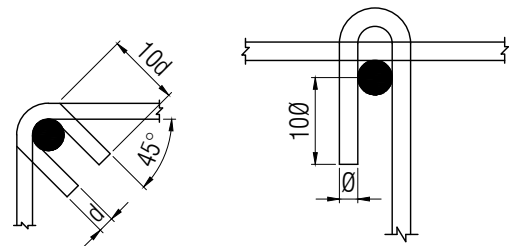
FOR 135° HOOK FOR 180° HOOK
