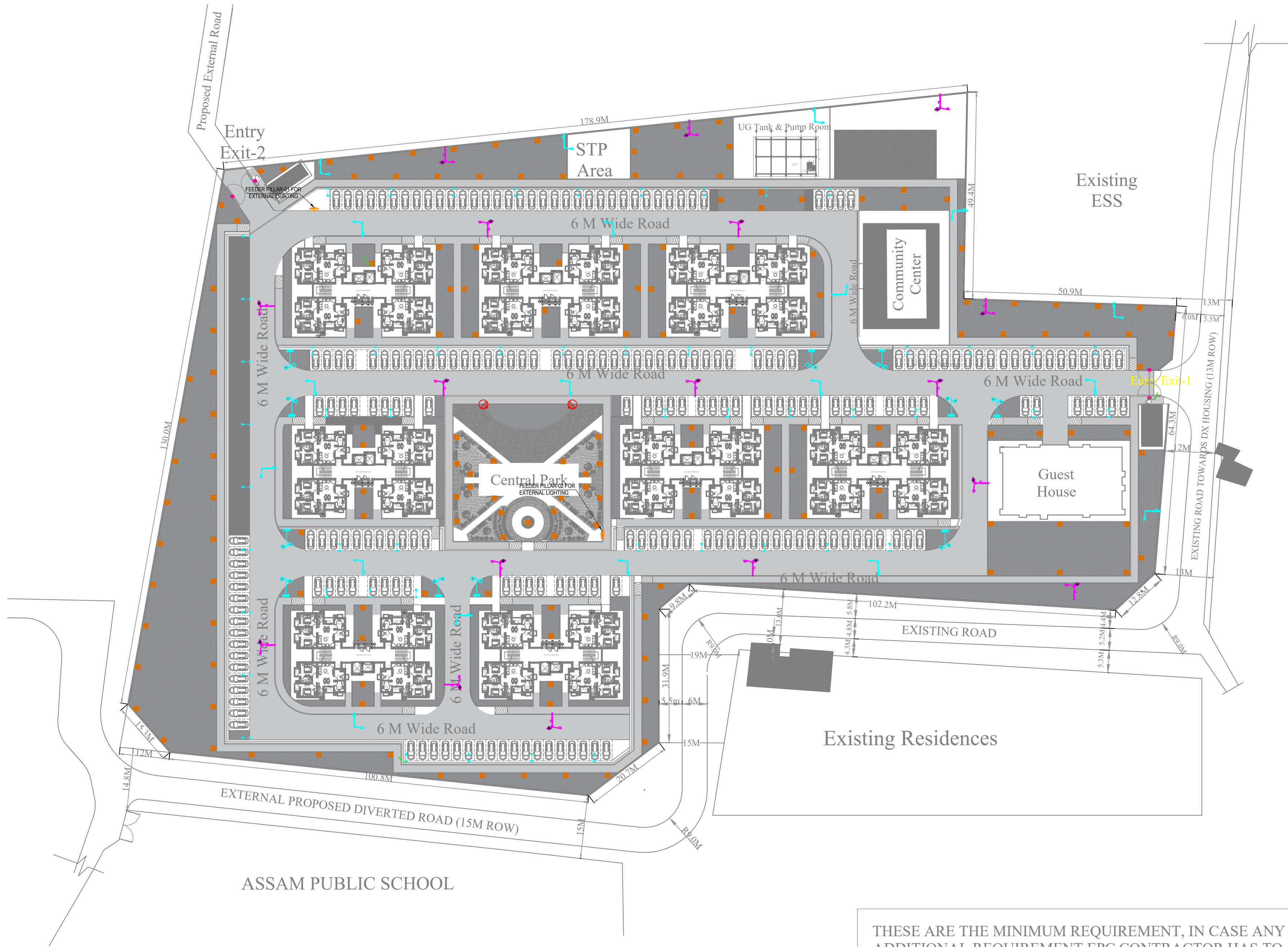
SITE LAYOUT
