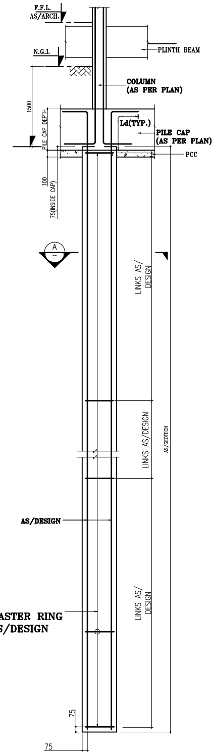
TYPICAL ELEVATION OF PILE (600MM DIA)
