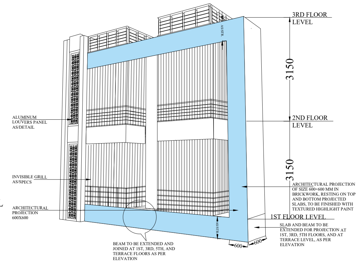
PROJECTION DETAIL
