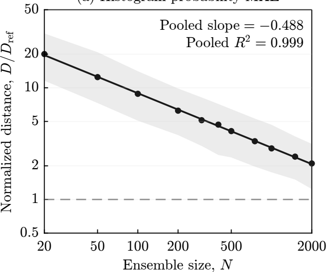
(a) Histogram-probability MAE
