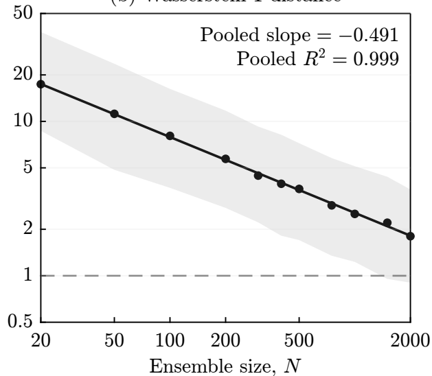
(b) Wasserstein-1 distance
