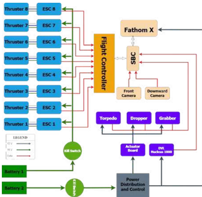
Circuit Diagram
