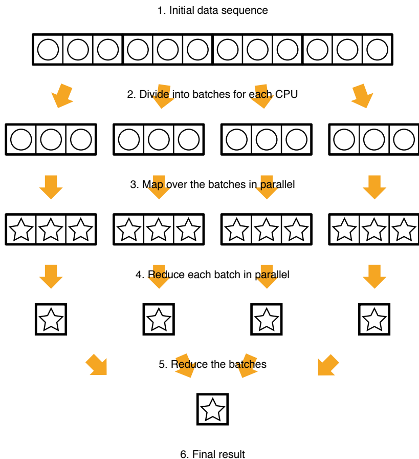
Figure 18.4: parallelFoldMap algorithm
